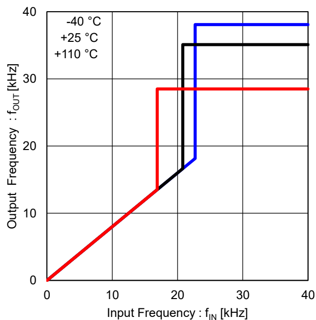
Figure 11. Output vs Input Frequency Characteristics
