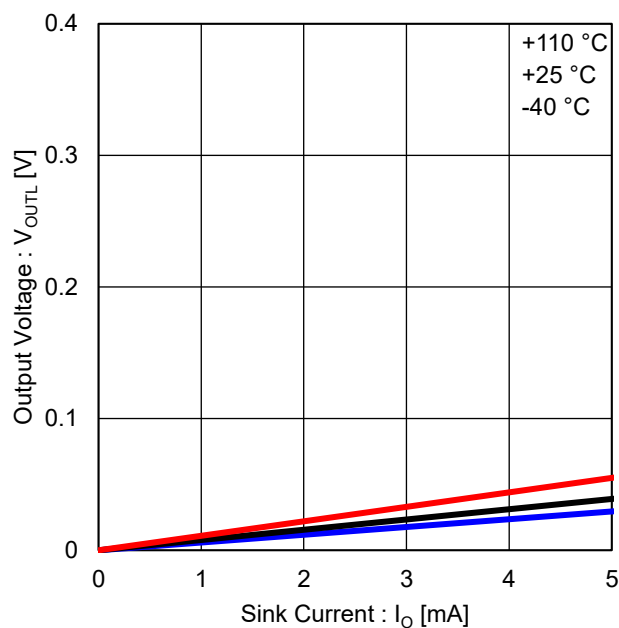
Figure 9. Output Low Voltage
