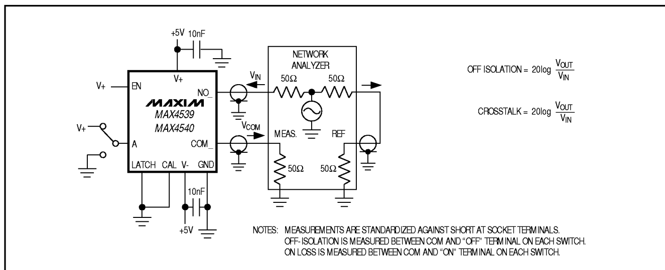
Figure 5. Off-Isolation/Crosstalk
