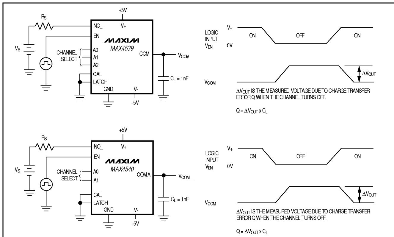
Figure 4. Charge Injection
