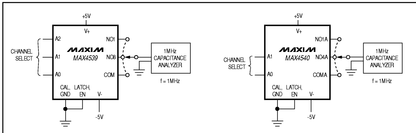
Figure 6. NO_/COM_ Capacitance
