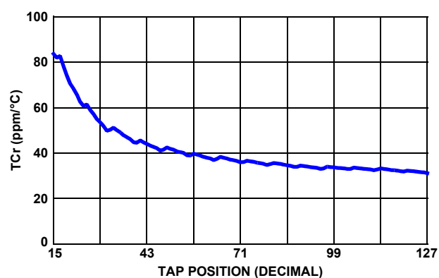
FIGURE 16. 50kΩ TCr vs TAP POSITION, V_{CC} = 3.3V
