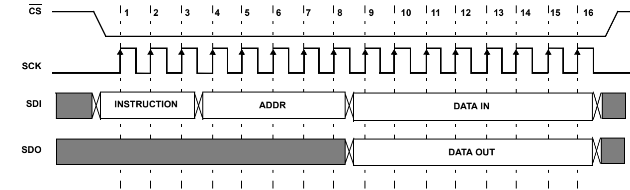
FIGURE 31. TWO BYTE READ INSTRUCTION
