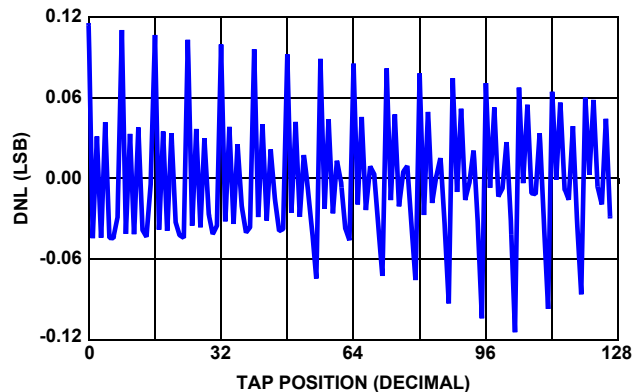
FIGURE 3. 10kΩ DNL vs TAP POSITION, V_{CC} = 3.3V , +25^{\circ}C
