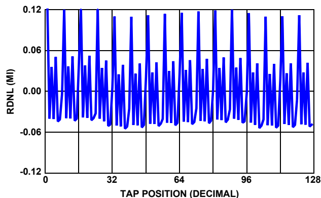
FIGURE 7. 10kΩ RDNL vs TAP POSITION, V_{CC} = 3.3V , +25^{\circ}C
