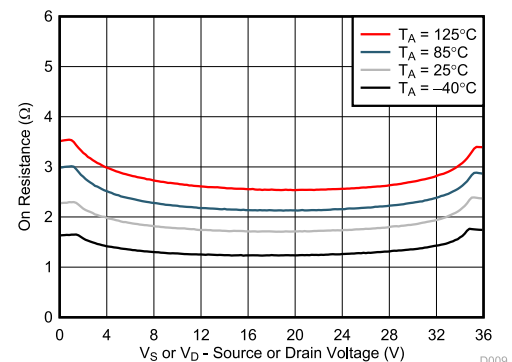
Figure 7-6. On-Resistance vs Temperature V_{DD} = 36\text{ V}, V_{SS} = 0\text{ V}
