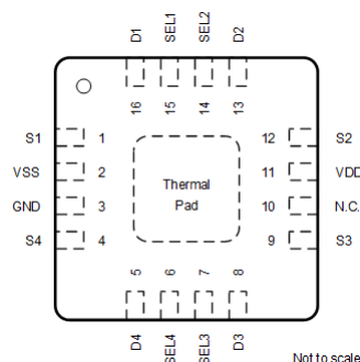
Figure 6-2. RUM Package 16-Pin WQFN Top View
