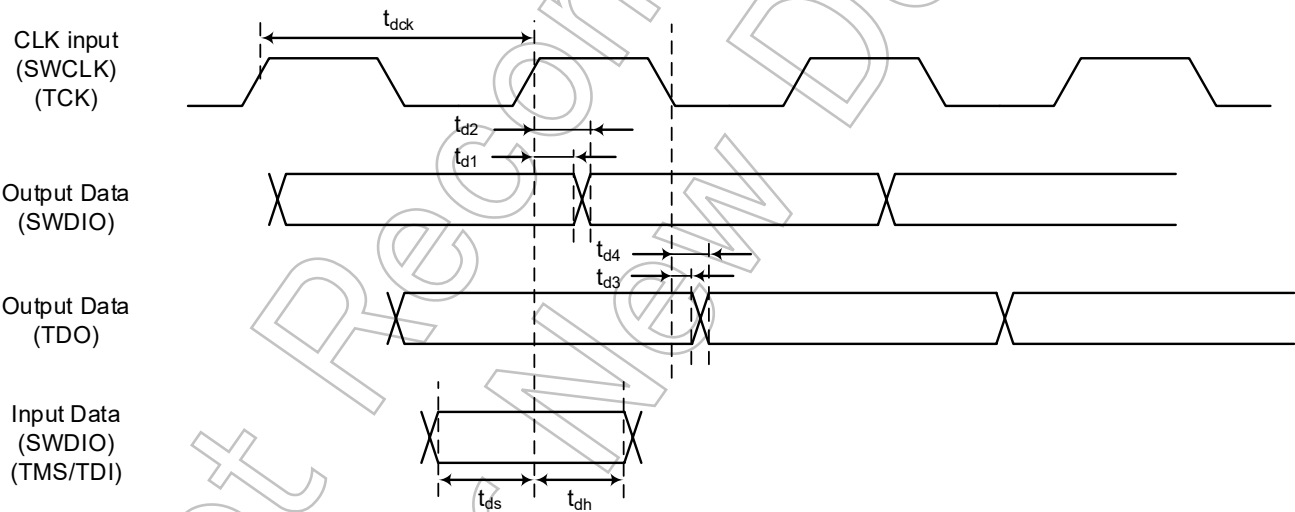
Figure 7.6 JTAG/SWD waveform
