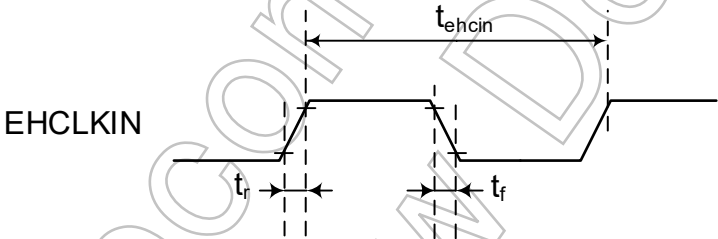
Figure 7.9 External clock input waveform
