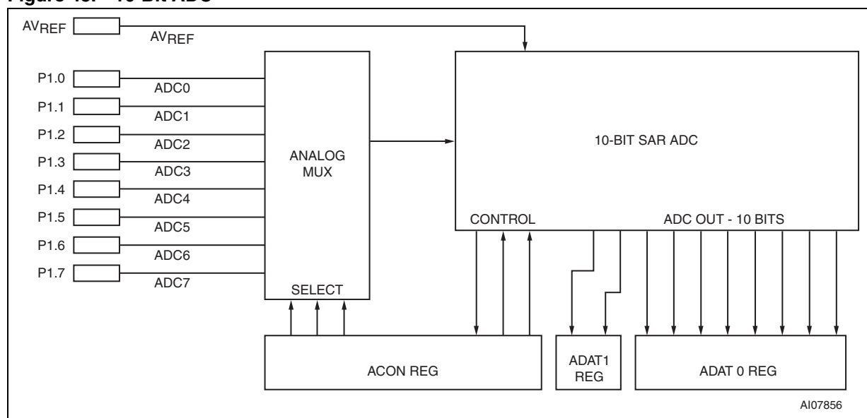
Figure 45. 10-Bit ADC
