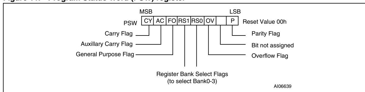
Figure 11. Program Status Word (PSW) register
