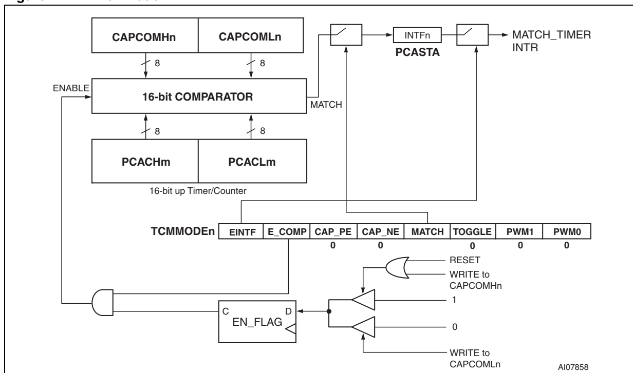
Figure 47. Timer mode
