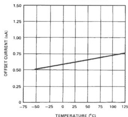
OFFSET CURRENT vs TEMPERATURE
