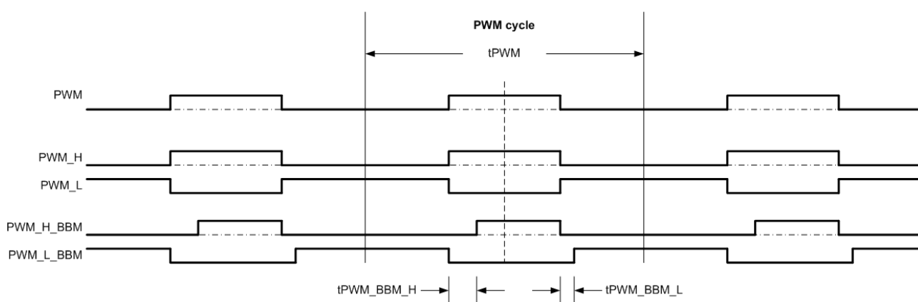
Figure 31: BBM Timing
