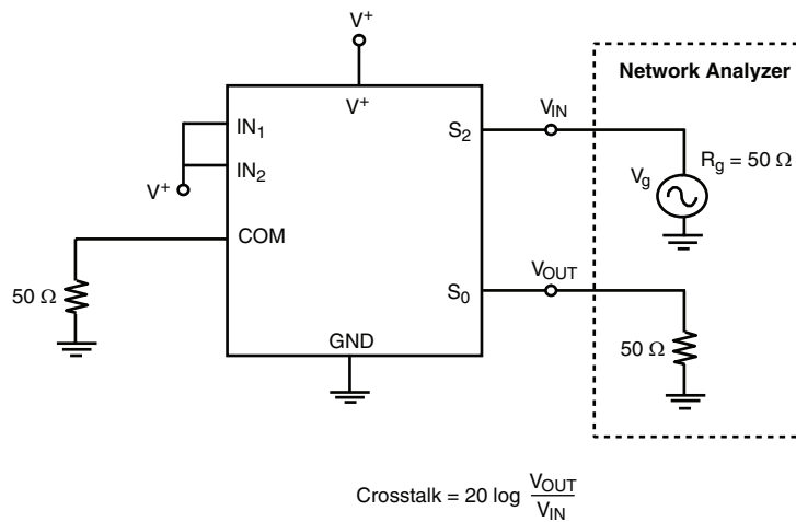
Figure 5. Crosstalk
