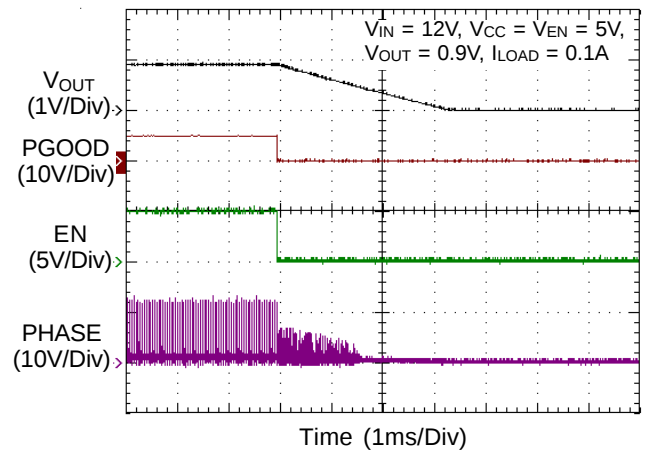
Power Off from V_{\text{IN}}
