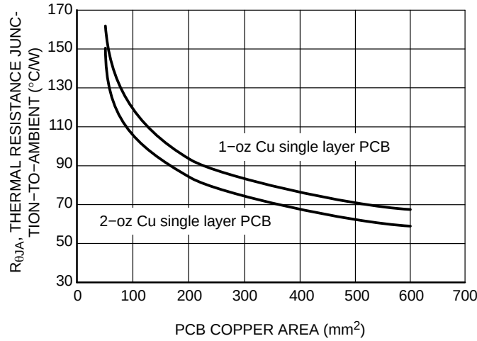
Figure 20. R_{\theta\text{JA}} vs. Copper Area
