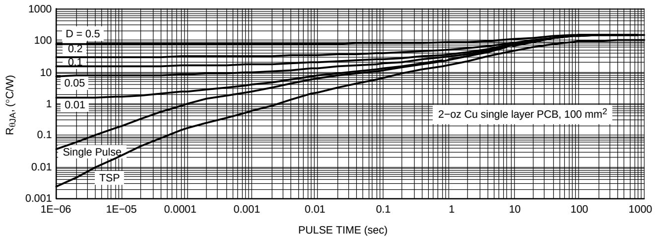
Figure 21. R_{\theta\text{JA}} vs. Duty Cycle
