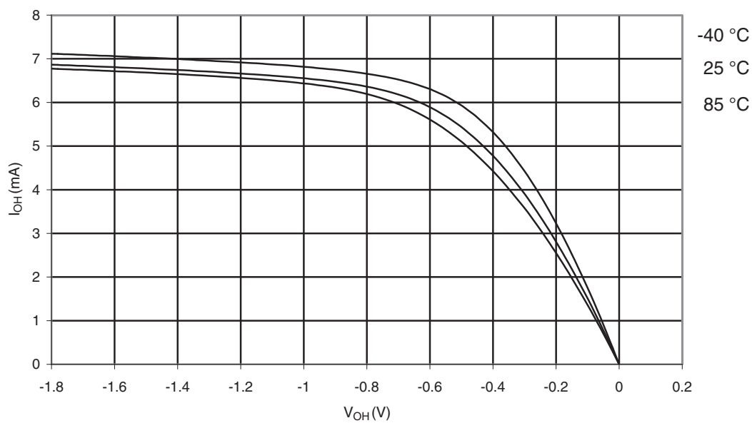
Figure 29-83. ATmega3290P: I/O Pin Source Current vs. Output Voltage, Port B ( V_{CC}=1.8V )
