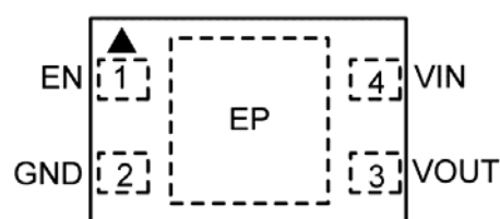
Top View 4-Pin 1.2mm × 1.6mm Thin MLF ® (MT)
