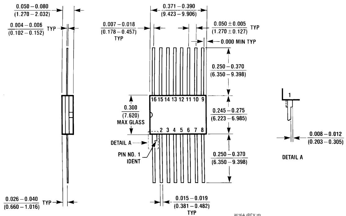
16-Lead Ceramic Flatpack NS Package Number W16A
