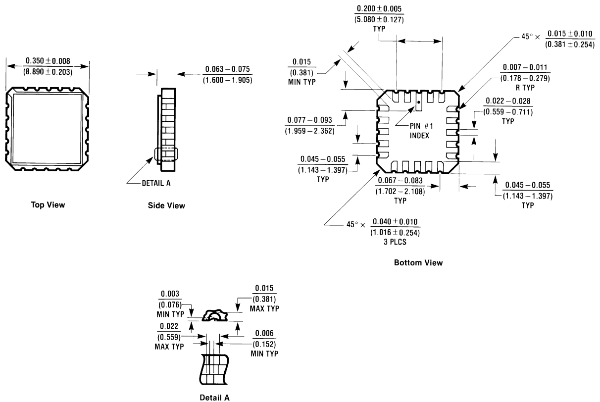
20-Lead Ceramic Leadless Chip Carrier NS Package Number E20A
