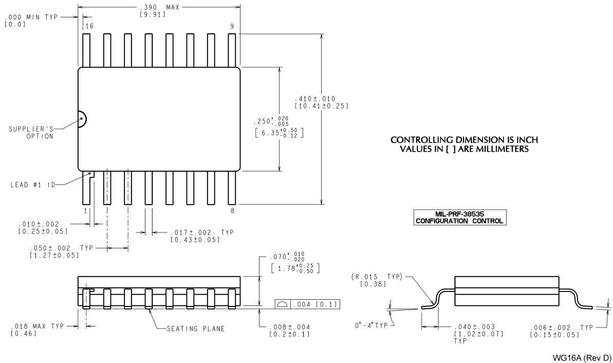
16-Lead Ceramic SOIC NS Package Number WG16A
