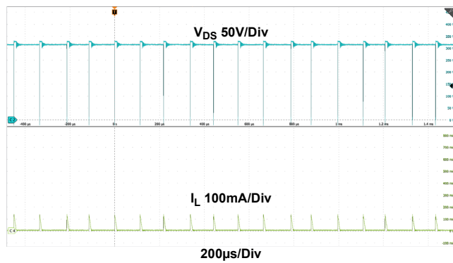
Figure 14. Light-Load Operation
