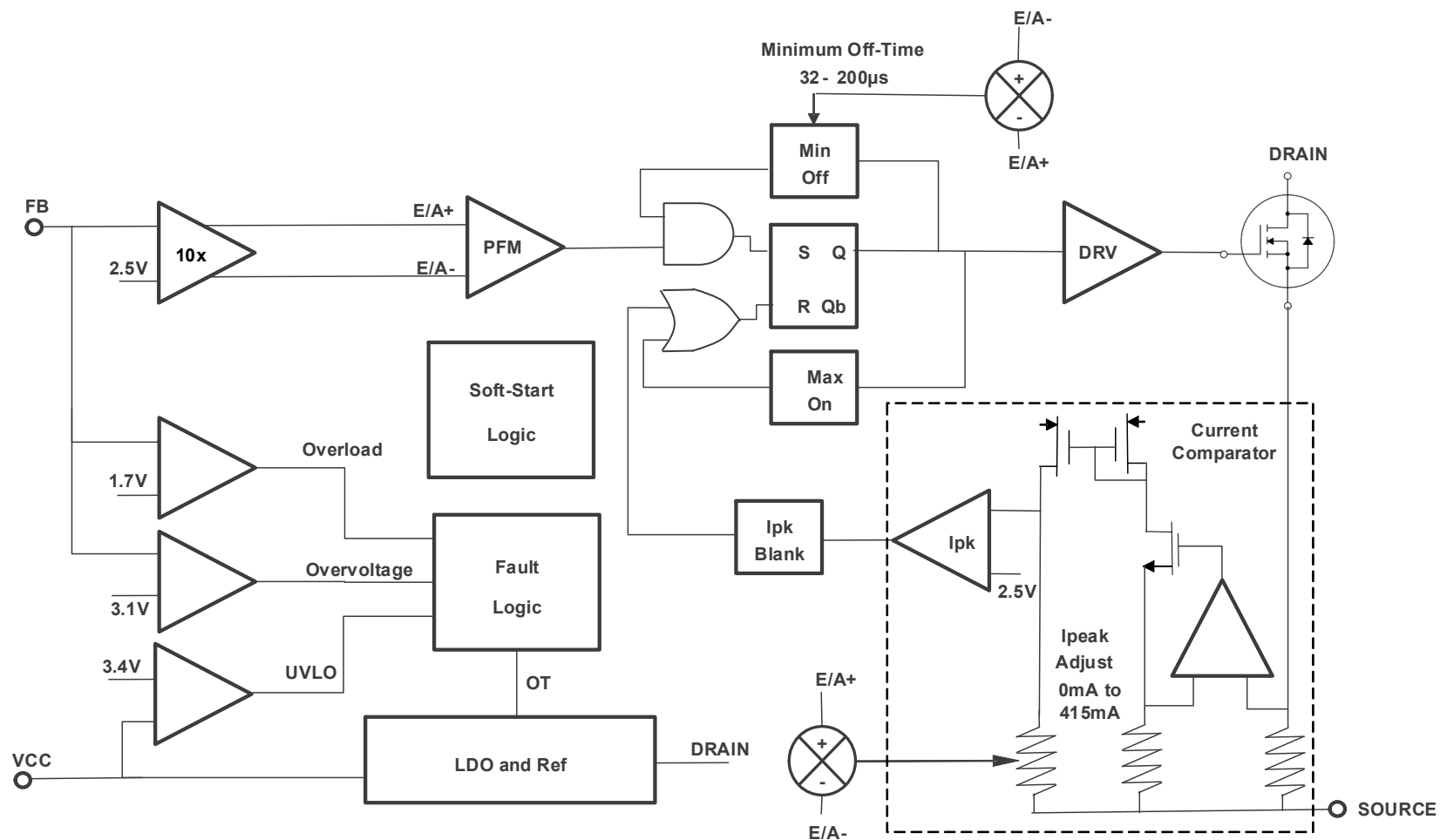
Figure 2. Block Diagram of RAA223011
