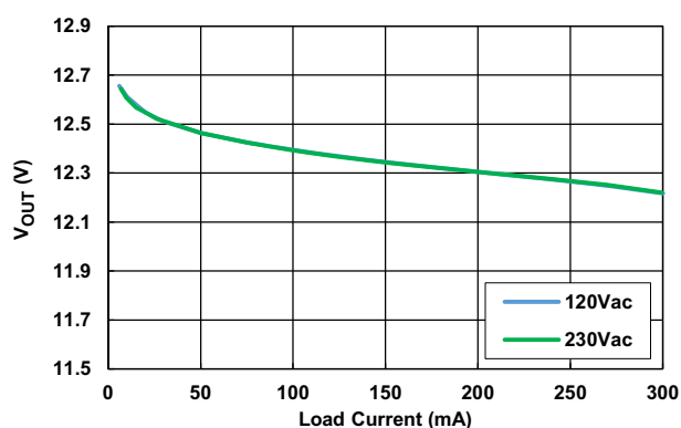
Figure 20. Load Regulation
