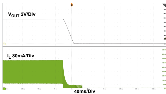
Figure 12. Shutdown
