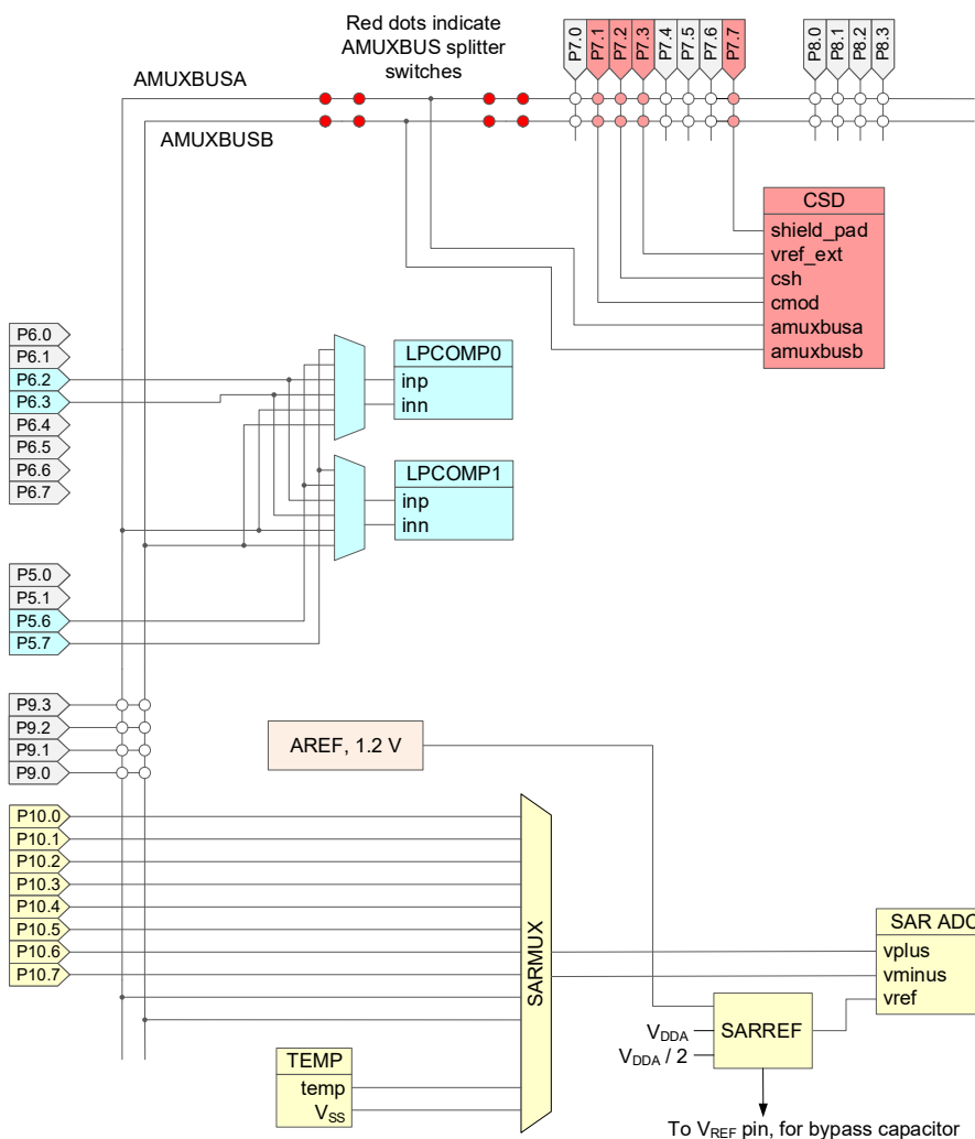
Figure 6. Analog Subsystem
