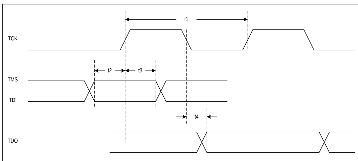
Figure-30 JTAG Interface Timing
