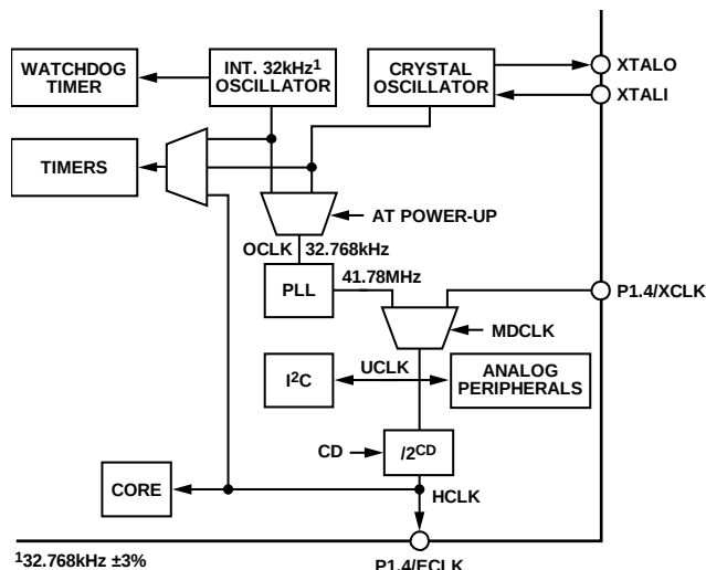
Figure 34. Clocking System
