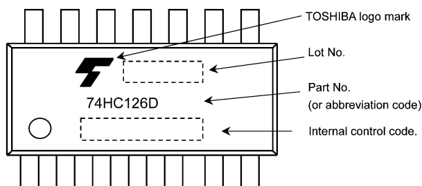
74HC126D
