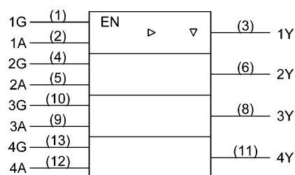
74HC126D
