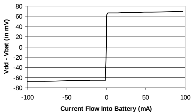
Headroom vs Battery Current
