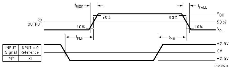
FIGURE 1. Propagation Delays
