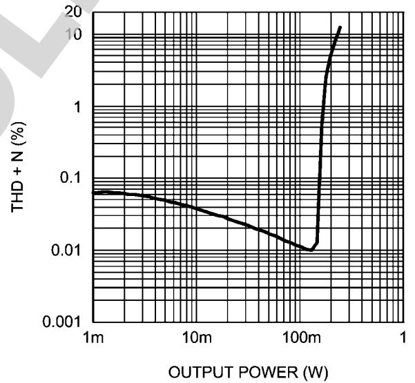
THD+N vs Output Power V_{DD} = 4.2V , R_L = 32\Omega , f = 1kHz One channel enabled
