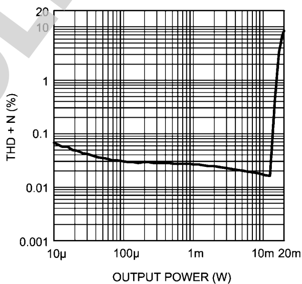
THD+N vs Output Power V_{DD} = 1.8V , R_L = 32\Omega , f = 1kHz One channel enabled
