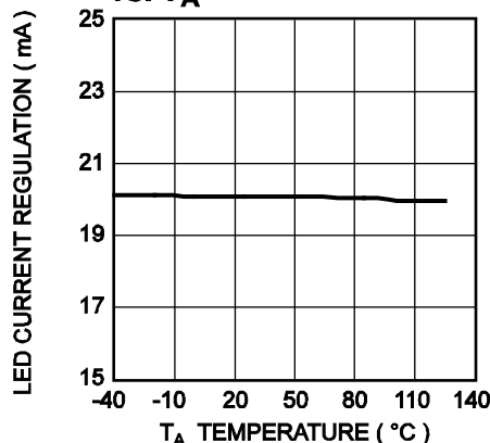
LED Current Regulation vs. T_A
