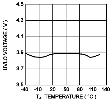
UVLO vs. T_A
