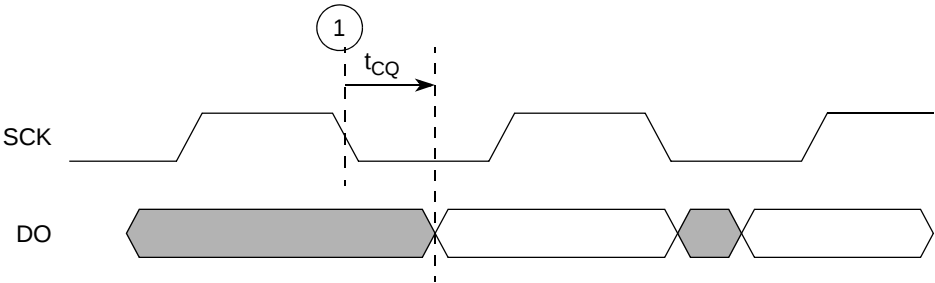
Figure 43. QuadSPI output timing diagram
