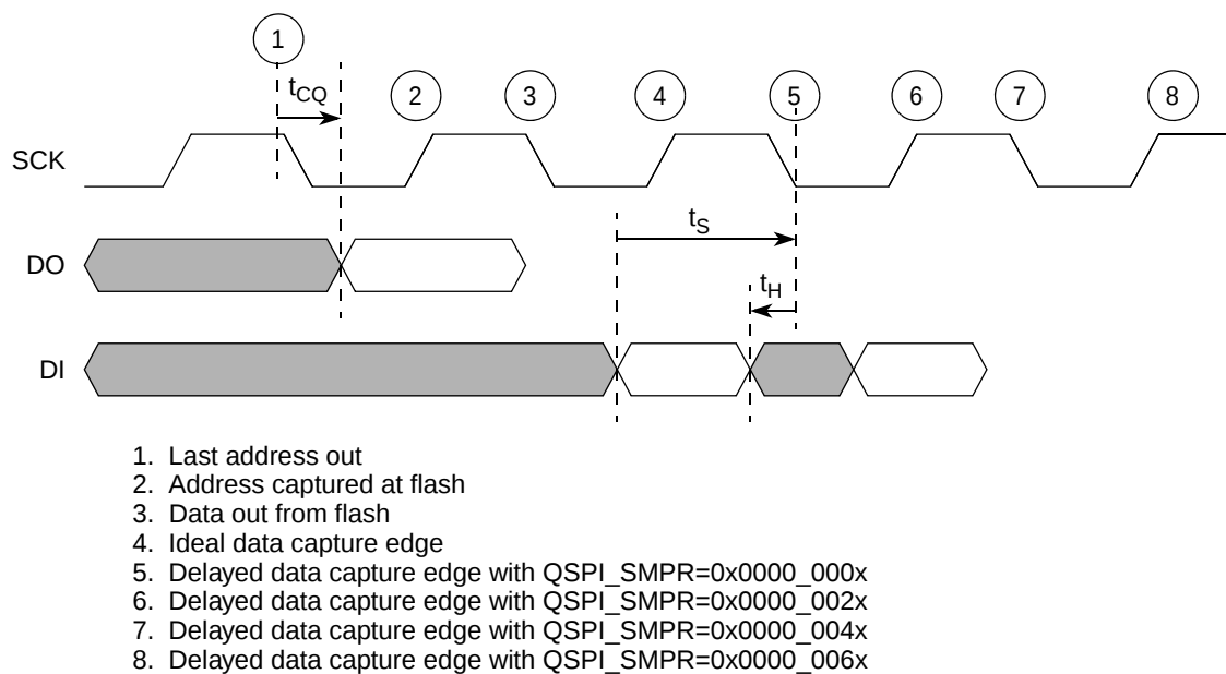
Figure 44. QuadSPI input timing diagram
