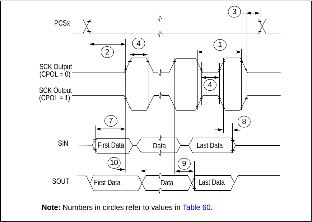
Figure 38. DSPI modified transfer format timing — master, CPHA = 0
