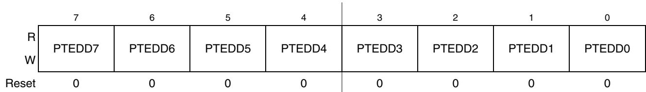
Figure 6-28. Data Direction for Port E (PTEDD)
