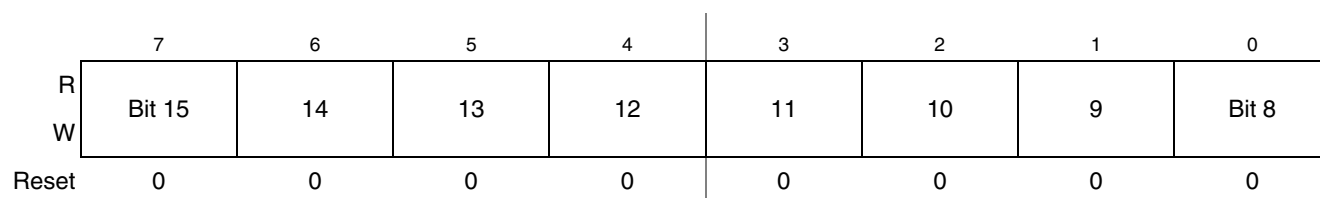
Figure 10-8. Timer x Counter Modulo Register High (TPMxMODH)
