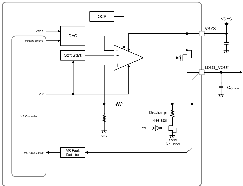
Figure 5-9. LDO1 Block Diagram
