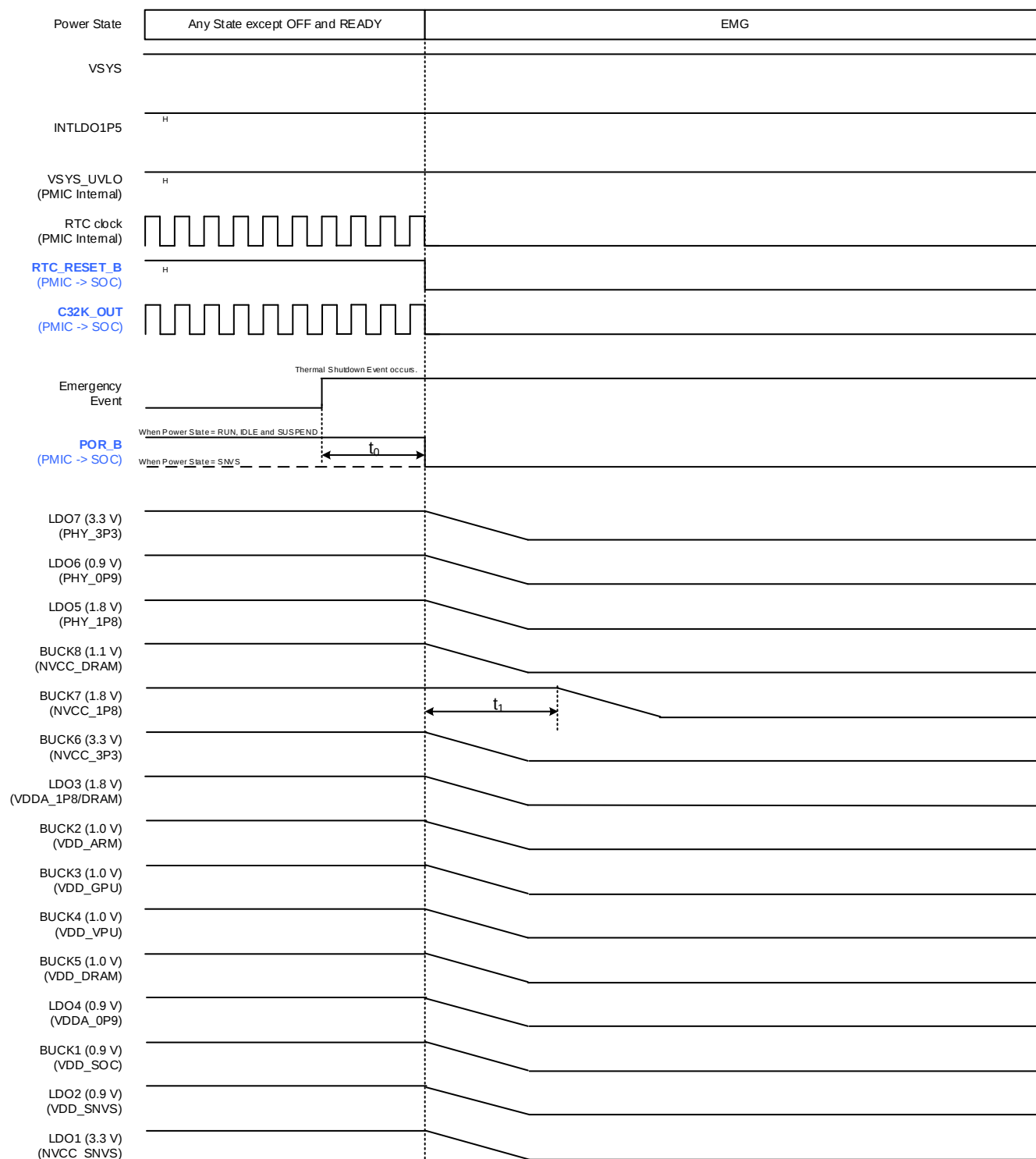
Figure 3-29. Emergency Shutdown
