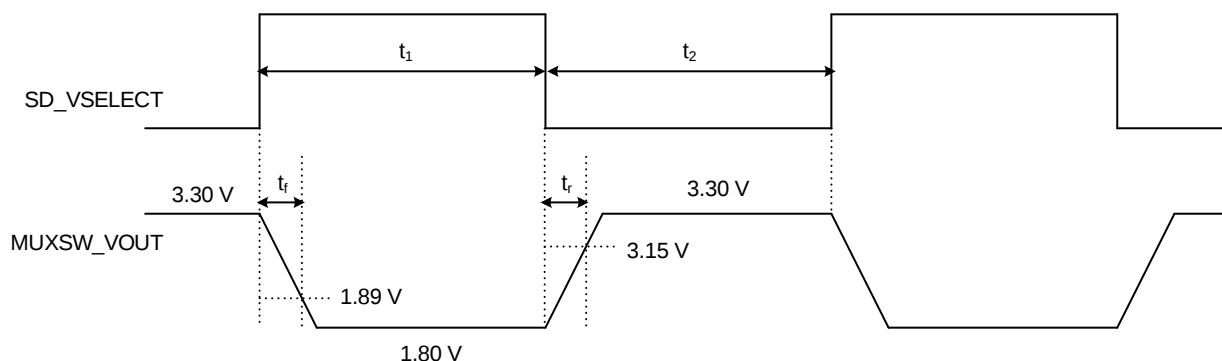
Figure 5-19. MUXSW Sequence
