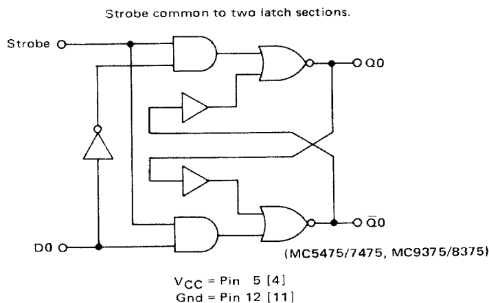
CIRCUIT SCHEMATIC 1/4 OF CIRCUIT SHOWN
