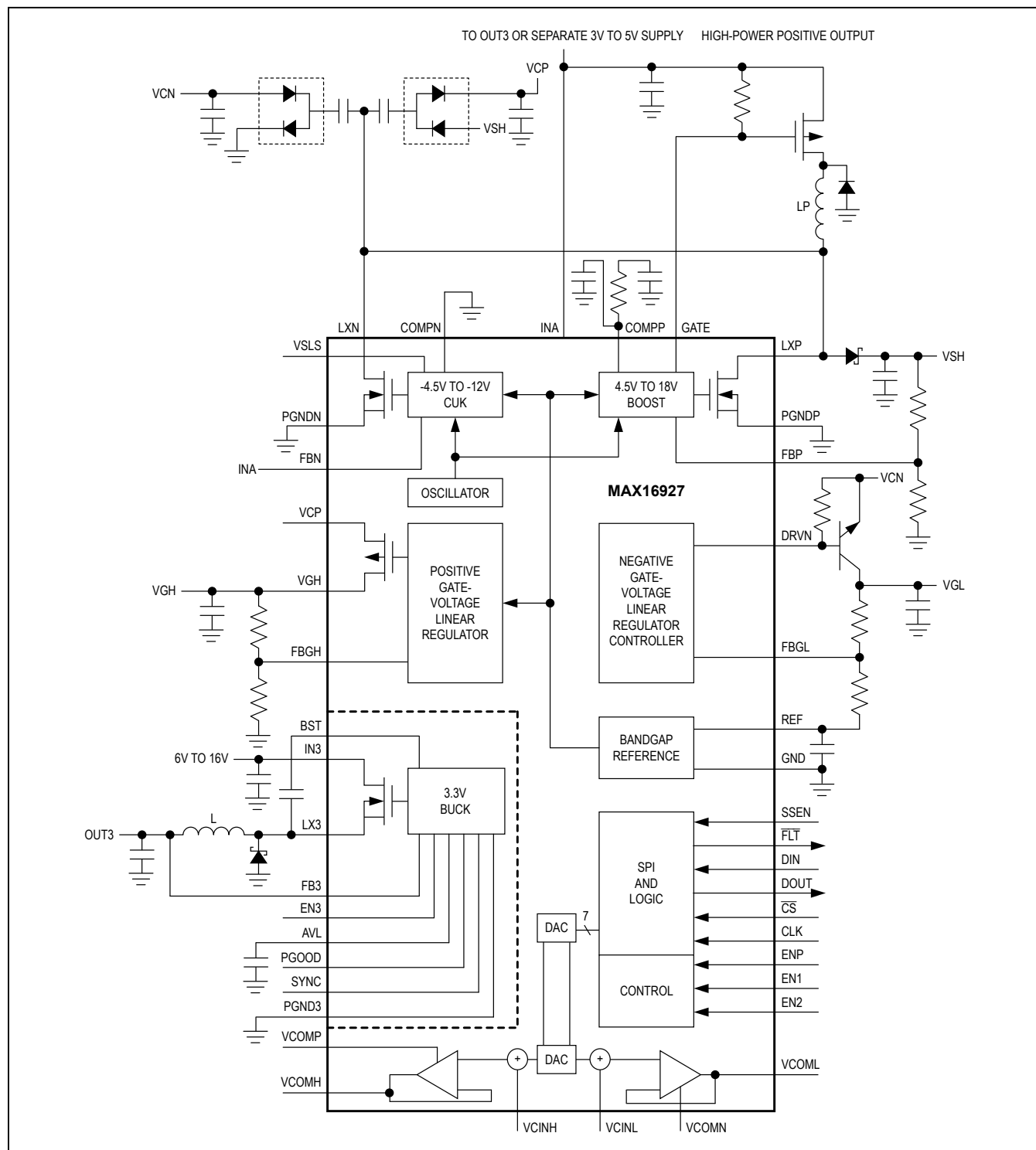
Figure 10. Typical High-Power Operating Circuit
