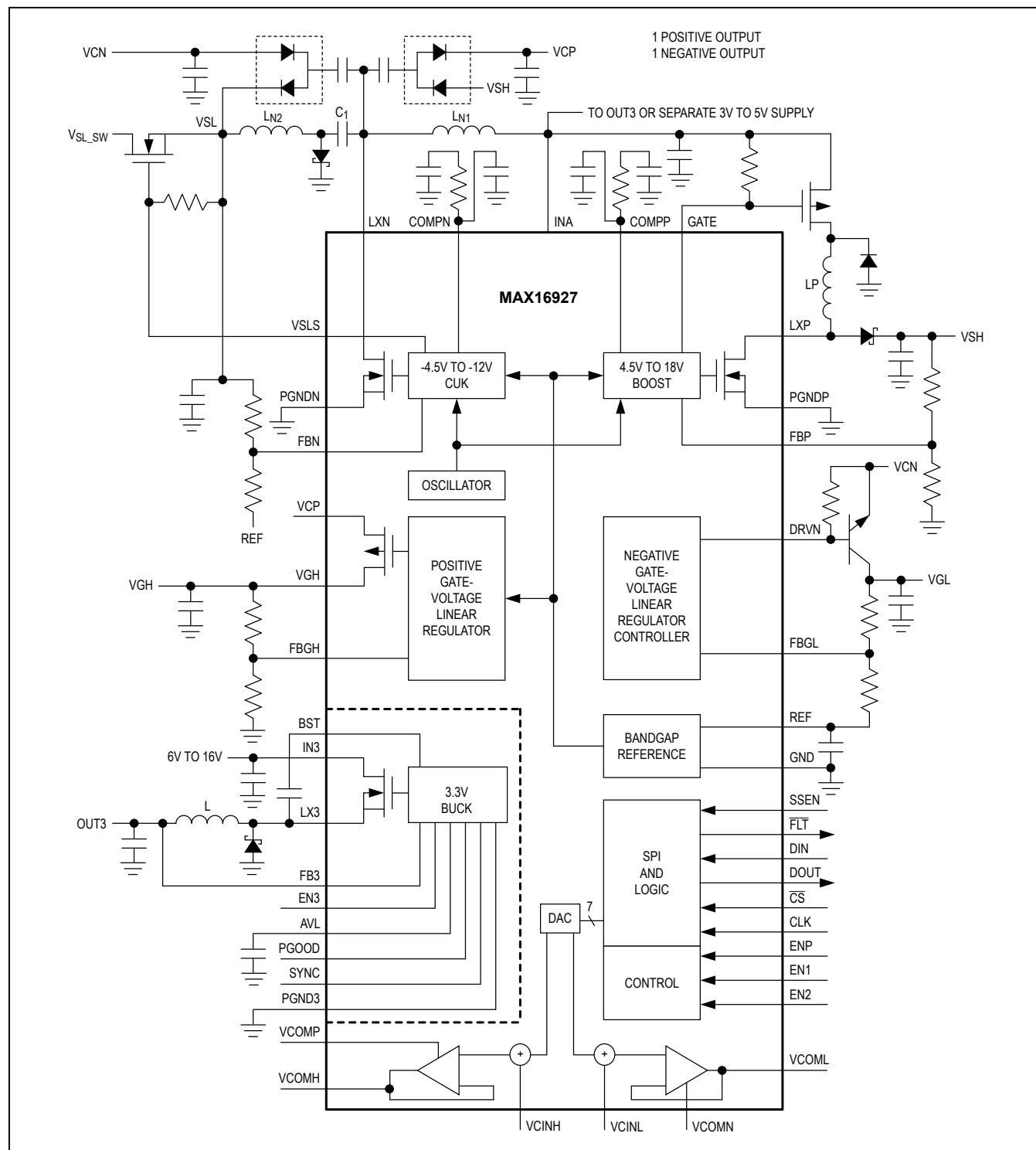
Figure 9. Typical Operating Circuit
