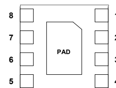
NJU77903KW2 PIN CONFIGURATION
