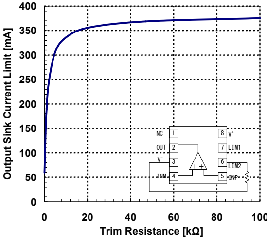
Output Sink Current Limit vs. Current Limit Trim Resistance V^+/V^- = 30V/0V , T_a = 25^\circ C , R_L = 1\Omega
