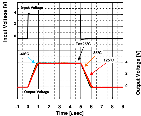
Pulse Response
