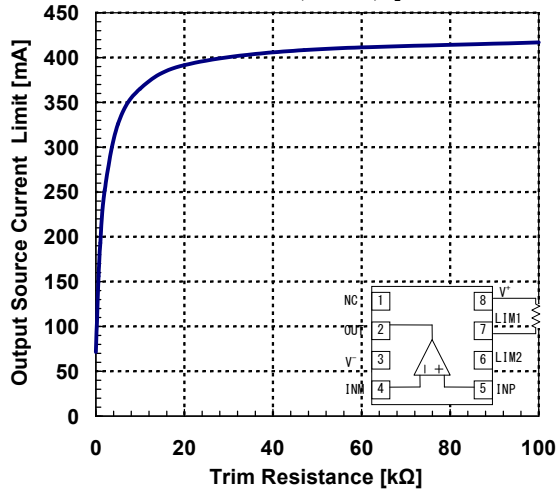
Output Source Current Limit vs. Current Limit Trim Resistance V^+/V^- = 30V/0V , T_a = 25^\circ C , R_L = 1\Omega
