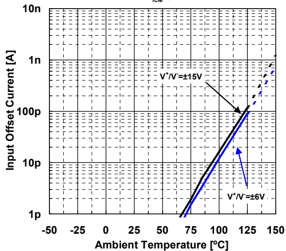
Input Offset Current vs. Temperature V_{ICM} = 0V
