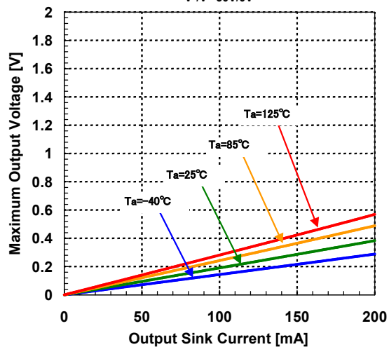
Maximum Output Voltage vs. Output Sink Current V^+/V^- = 30V/0V
