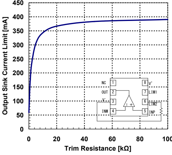
Output Sink Current Limit vs. Current Limit Trim Resistance V^+/V^- = 12V/0V , T_a = 25^\circ C , R_L = 1\Omega
