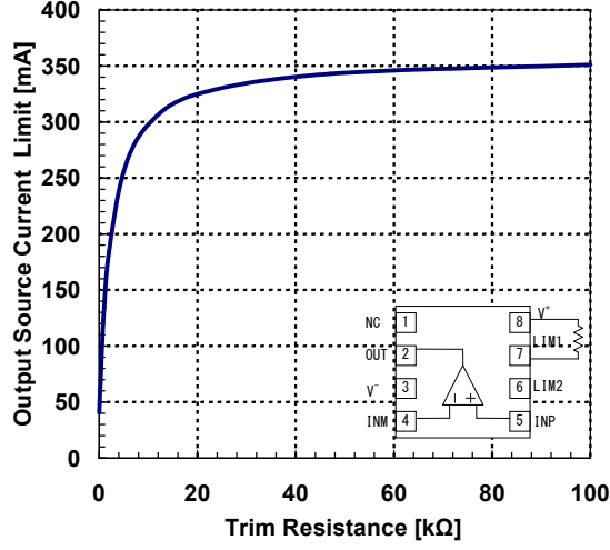
Output Source Current Limit vs. Current Limit Trim Resistance V^+/V^- = 12V/0V , T_a = 25^\circ C , R_L = 1\Omega
