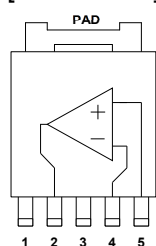
NJU77903DL3 PIN CONFIGURATION
