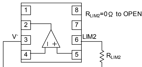
Figure 2-2: Output Sink Current Limit Trim
