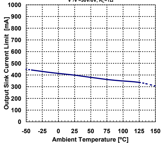
Output Sink Current Limit vs. Temperature V^+/V=30\text{V}/0\text{V} , R_L=1\Omega
