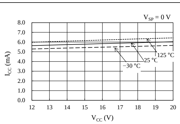
Figure 14-3. Logic Supply Current, I_{CC} vs. VCC Pin Voltage, V_{CC}
