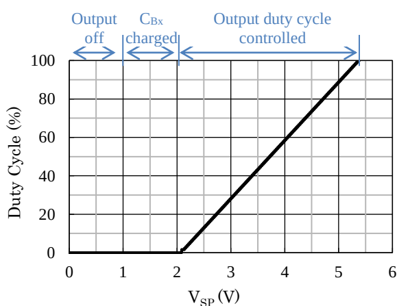
Figure 11-11. VSP Pin Voltage vs. Duty Cycle
