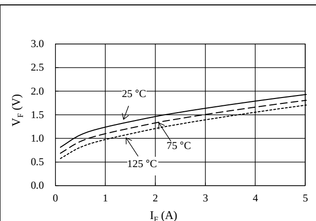
Figure 14-20. Freewheeling Diode V_F vs. I_F
