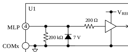
Figure 11-2. Internal Circuit Diagram of MLP Pin
