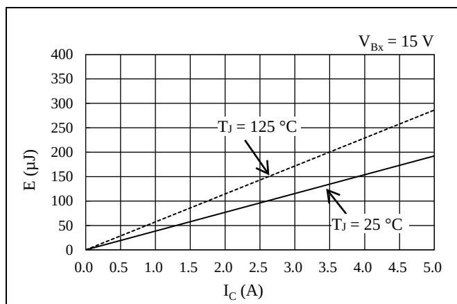
Figure 14-21. High-side Switching Loss
