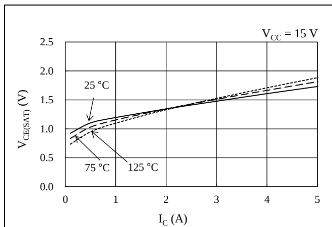
Figure 14-19. IGBT V_{CE(SAT)} vs. I_C
