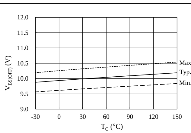
Figure 14-7. High-side Logic Operation Stop Voltage, V_{BS(OFF)} vs. T_C
