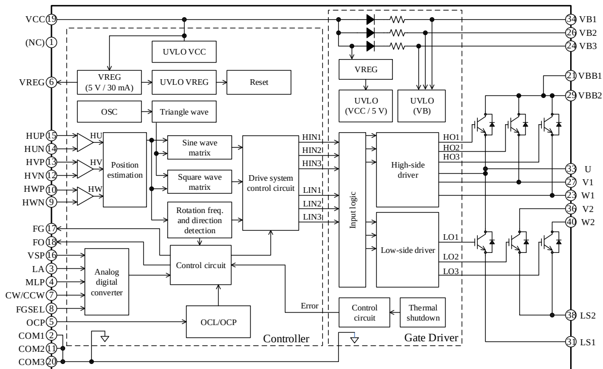
Figure 6-1. Block Diagram
