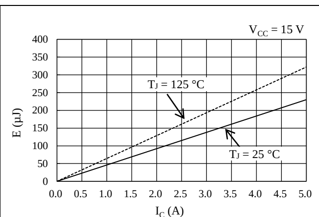
Figure 14-22. Low-side Switching Loss
