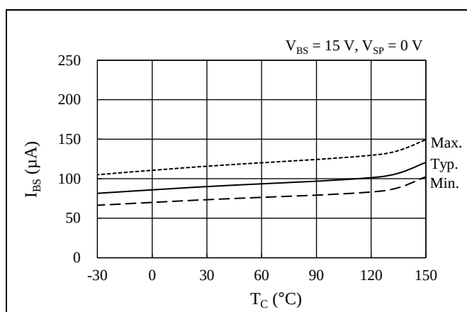
Figure 14-4. Logic Supply Current in 1-phase Operation ( V_{SP} = 0\text{ V} ), I_{BS} vs. T_C
