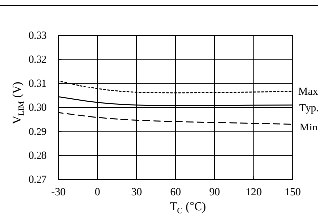
Figure 14-15. Current Limit Reference Voltage, V_{LIM} vs. T_C
