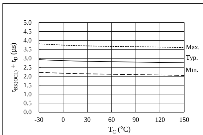
Figure 14-16. OCL Blanking Time, t_{BK(OCL)} + t_D vs. T_C
