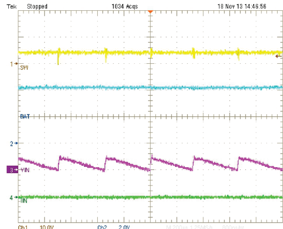
Figure 22. Boost Burst Mode During Light Load
