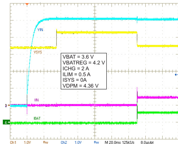
Figure 26. Startup, 4.2V
