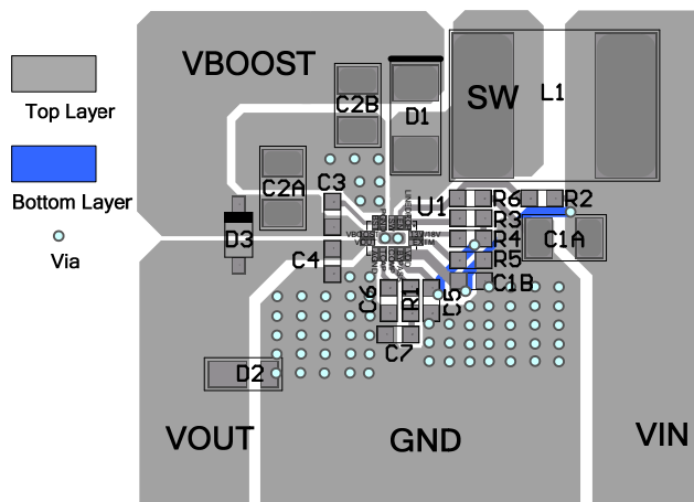
Figure 3: Layout Recommendation
