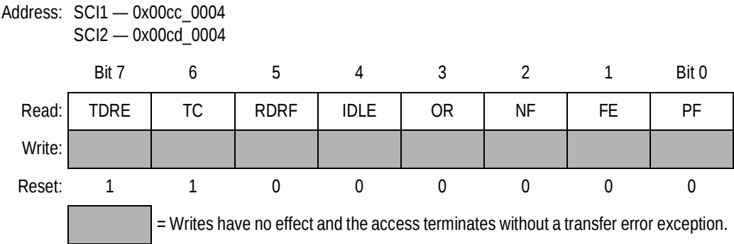
Figure 16-6. SCI Status Register 1 (SCISR1)
