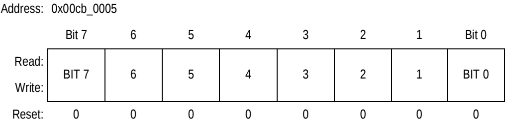
Figure 17-6. SPI Data Register (SPIDR)
