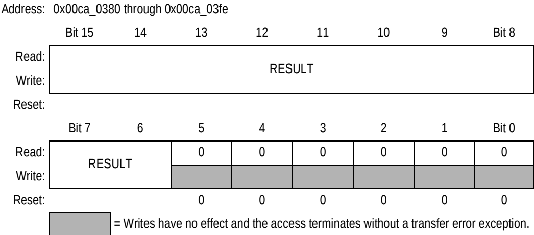
Figure 18-17. Left-Justified Unsigned Result Register (LJURR)
