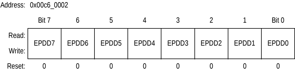
Figure 12-3. EPORT Data Direction Register (EPDDR)
