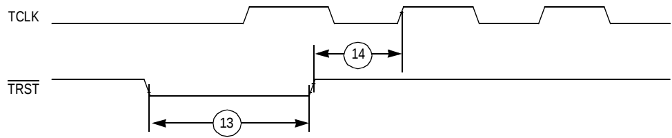
Figure 22-12. TRST Timing
