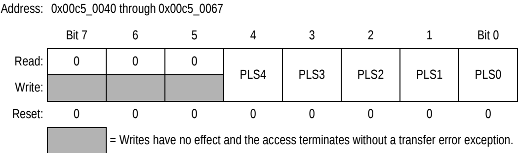
Figure 7-11. Priority Level Select Registers (PLSR0–PLSR39)
