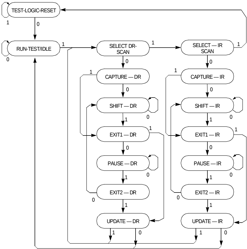
Figure 21-6. OnCE Controller
