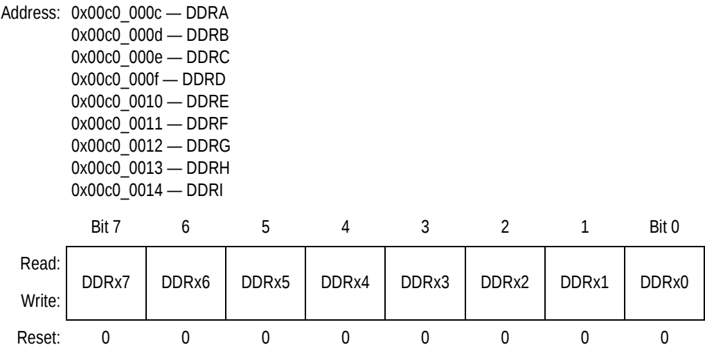
Figure 11-3. Port Data Direction Registers (DDRx)
