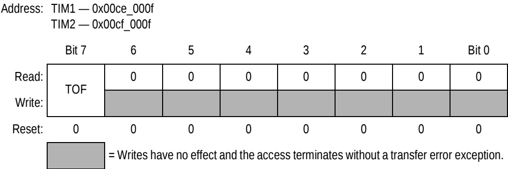
Figure 15-16. Timer Flag Register 2 (TIMFLG2)
