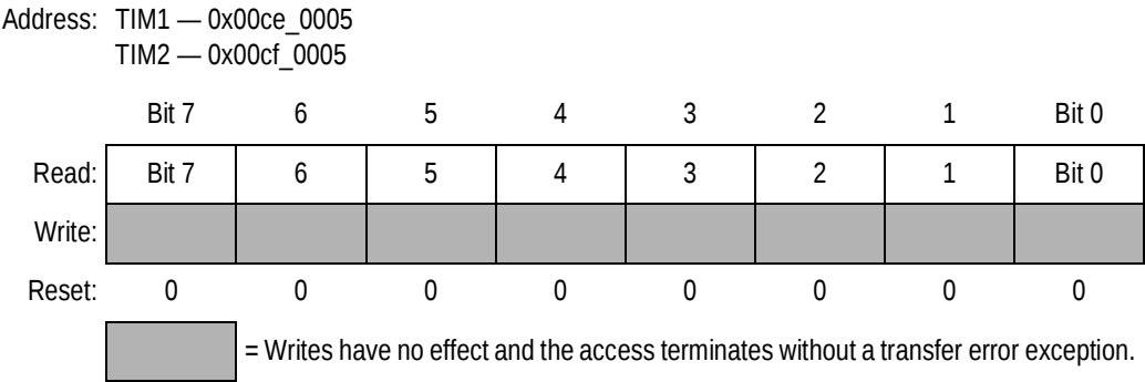
Figure 15-7. Timer Counter Register Low (TIMCNTL)
