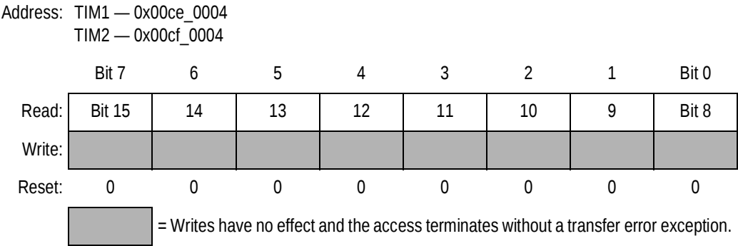
Figure 15-6. Timer Counter Register High (TIMCNTH)
