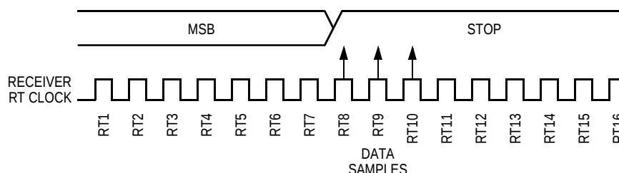
Figure 16-23. Slow Data
