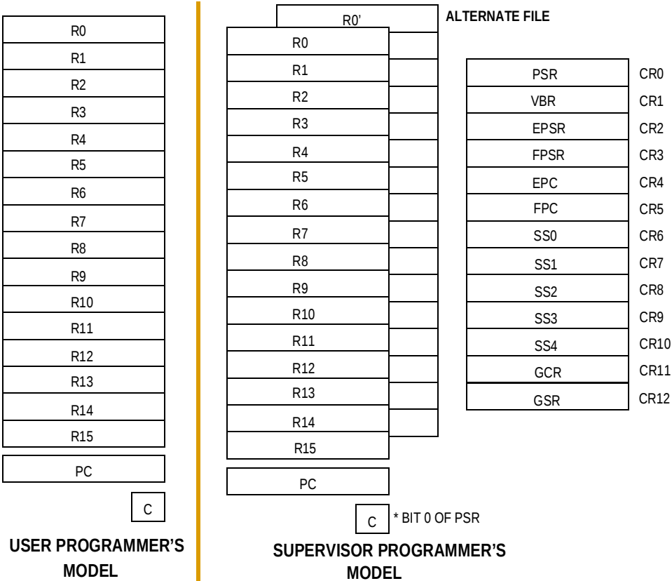
Figure 6-2. Programming Model
