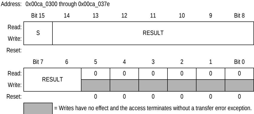
Figure 18-16. Left-Justified Signed Result Register (LJSRR)
