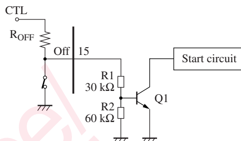
Figure 9. Off terminal peripheral circuit
