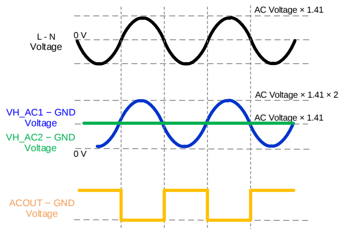
Figure 4. Double Voltage Rectification Waveform
