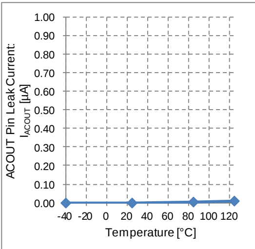
Figure 16. ACOU Pin Leak Current vs Temperature
