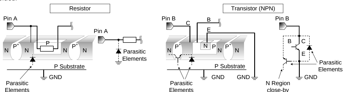
Figure 19. Example of IC Structure
