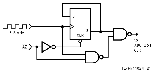
FIGURE 5. Switching between a Conversion with and without Auto-Zero when Using \overline{WR} Control
