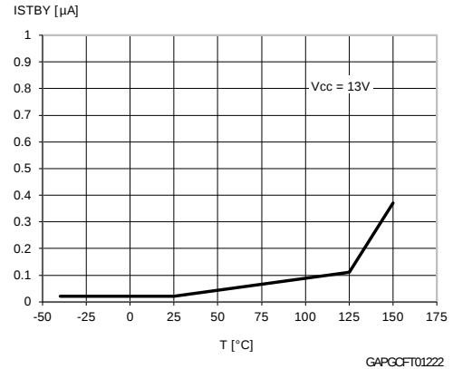
Figure 16: Standby current
