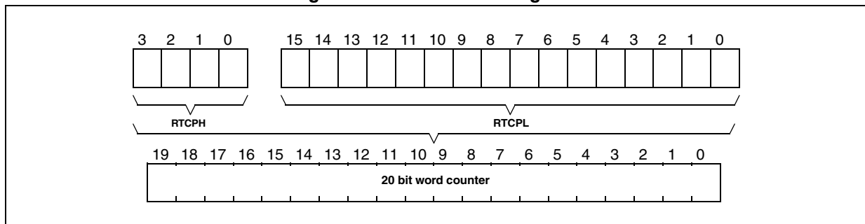
Figure 51. PRESCALER Register
