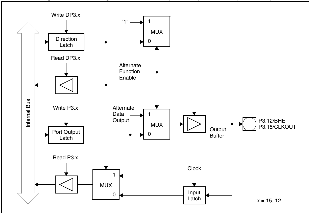
Figure 28. Block Diagram of Pins P3.15 (CLKOUT) and P3.12 ( \overline{\text{BHE}}/\overline{\text{WRH}} )
