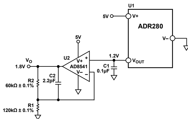
Figure 15. 1.8 V Reference
