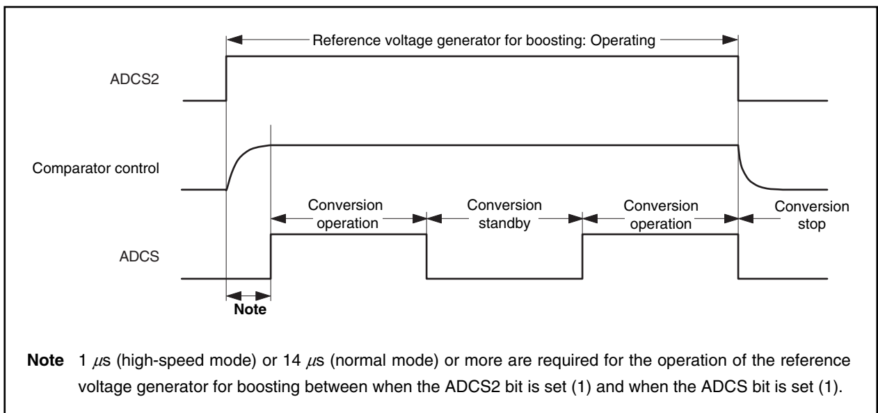
Figure 13-2. Operation Sequence
