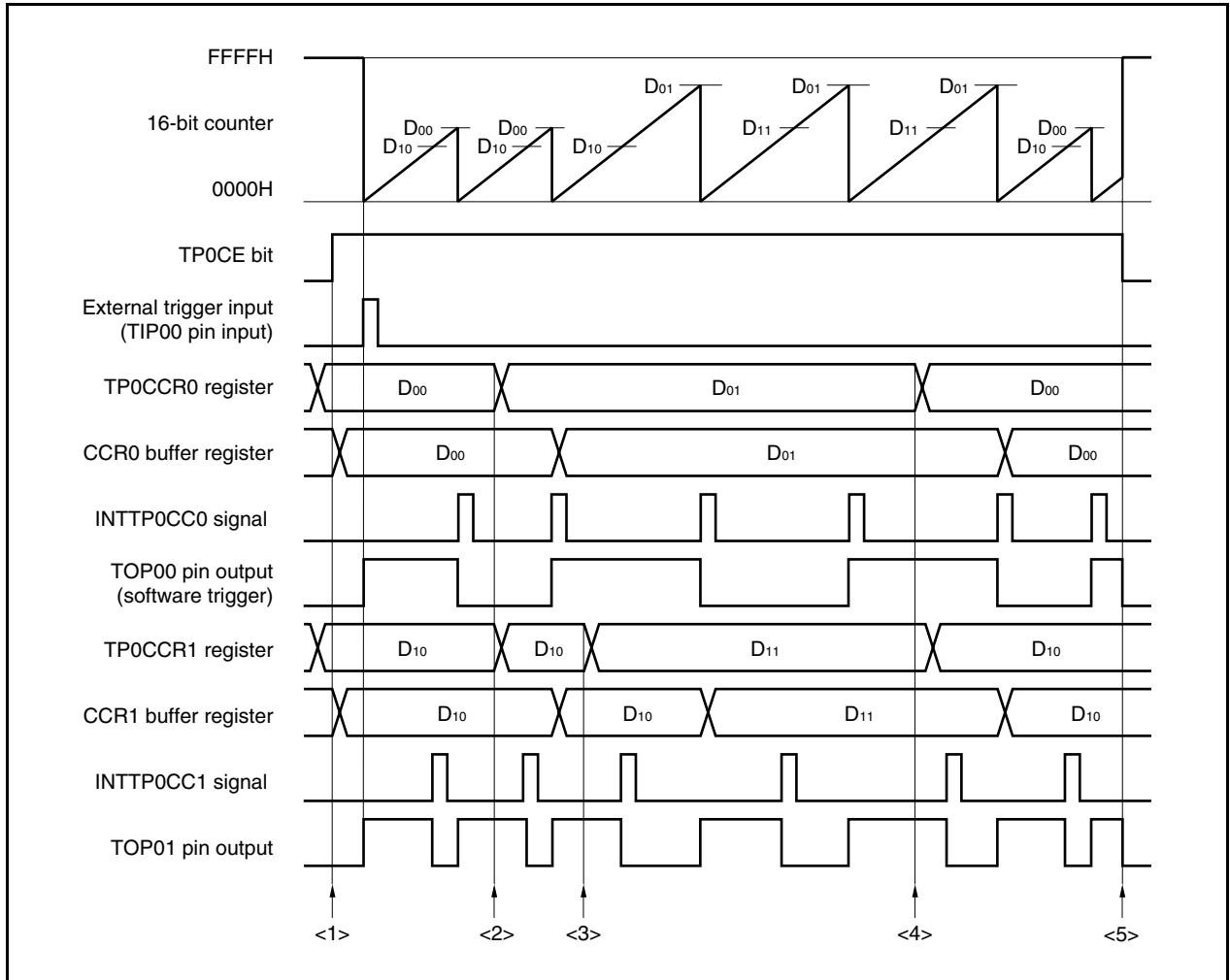
Figure 6-19. Software Processing Flow in External Trigger Pulse Output Mode (1/2)
