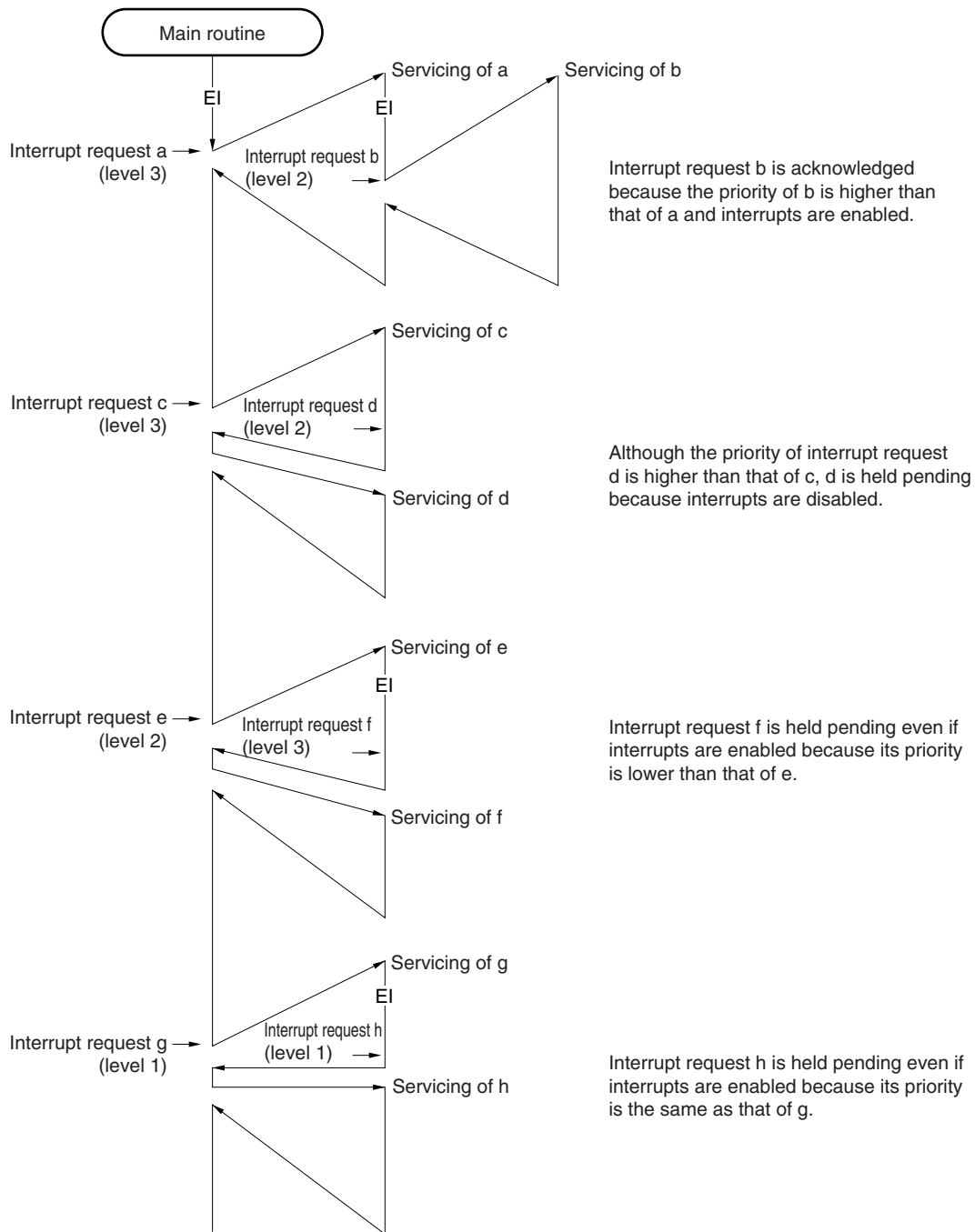
Figure 17-6. Example of Interrupt Nesting (1/2)
