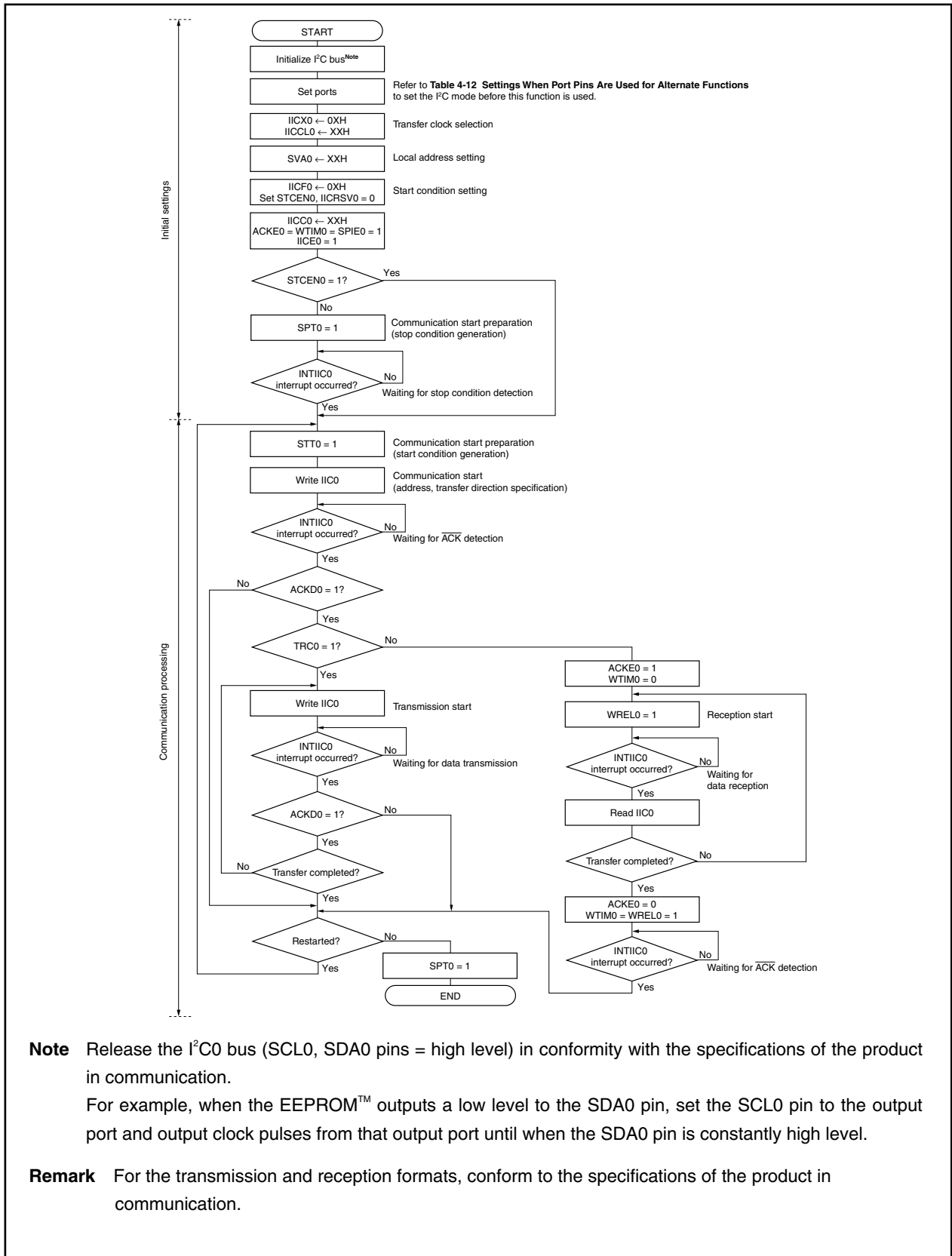
Figure 16-15. Master Operation in Single Master System
