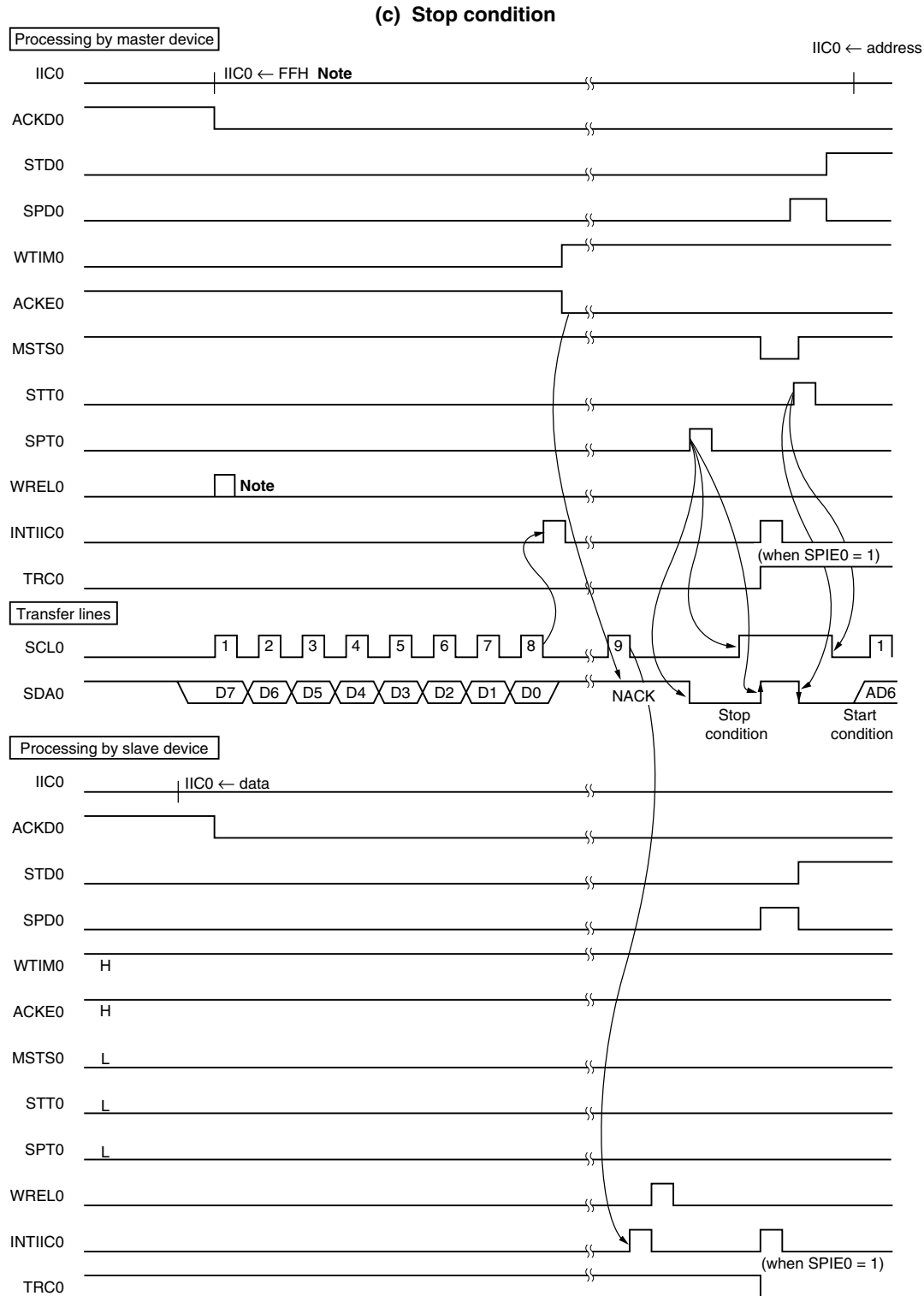
Figure 16-21. Example of Slave to Master Communication (When 8-Clock Wait for Master and 9-Clock Wait for Slave Are Selected) (3/3)
