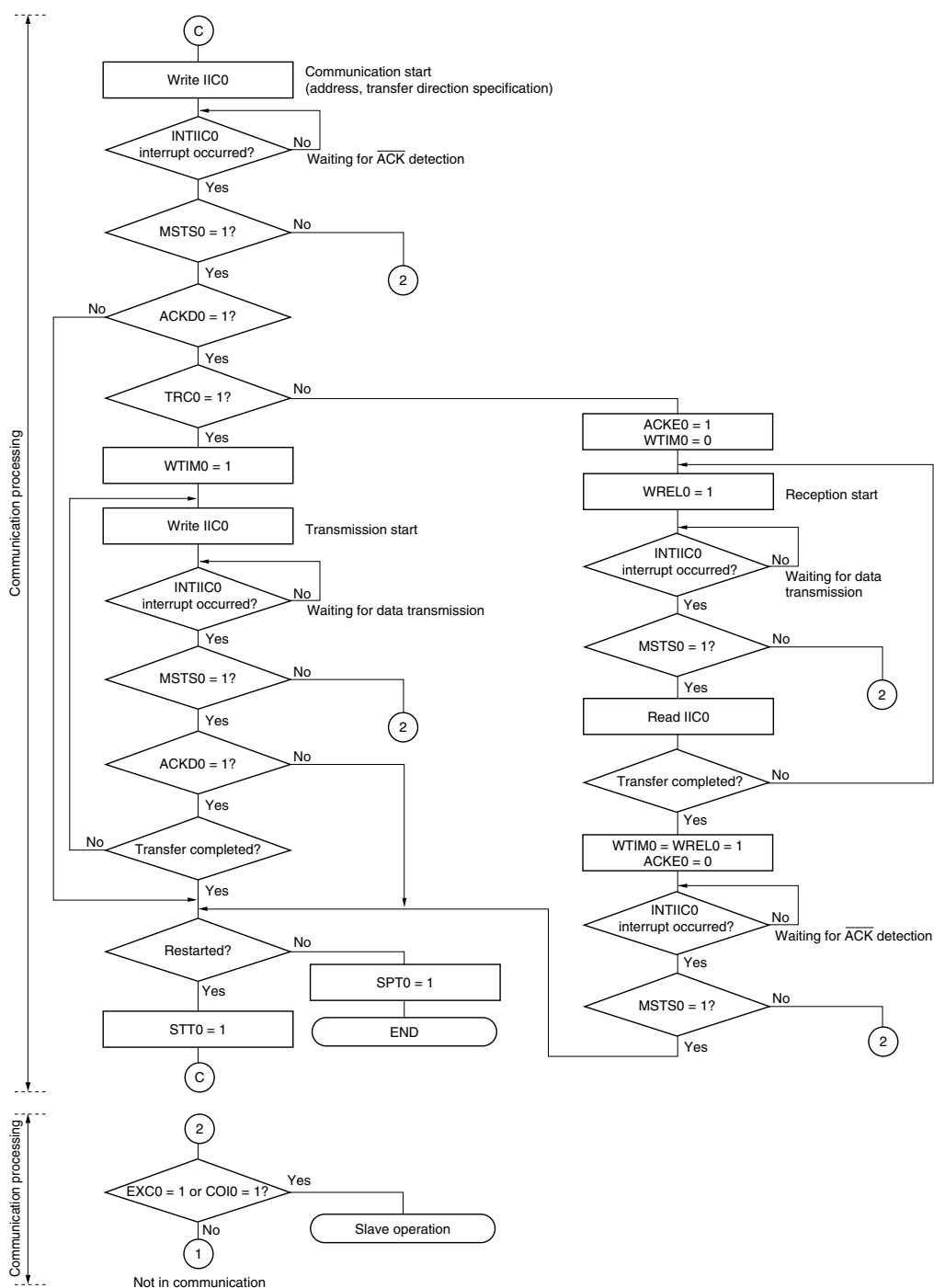
Figure 16-16. Master Operation in Multimaster System (3/3)
