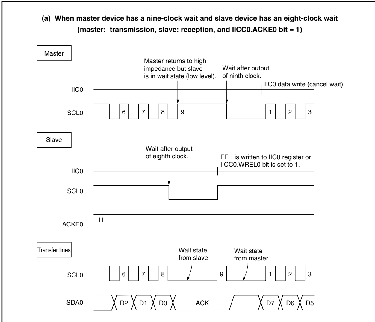
Figure 16-10. Wait State (1/2)
