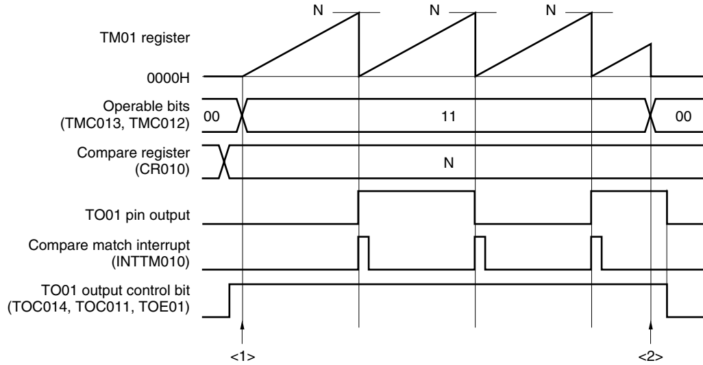
Figure 7-12. Example of Software Processing in External Event Counter Mode
