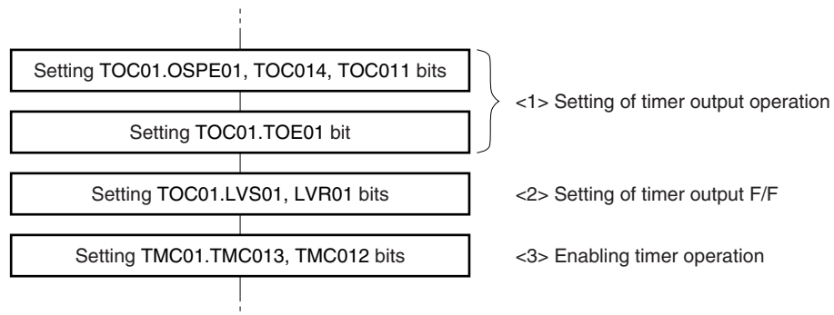
Figure 7-44. Example of Flow for Setting LVS01 and LVR01 Bits
