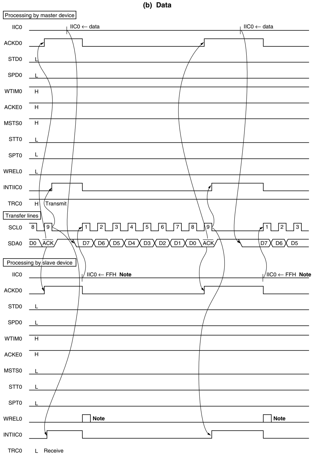
Figure 16-20. Example of Master to Slave Communication (When 9-Clock Wait Is Selected for Both Master and Slave) (2/3)
