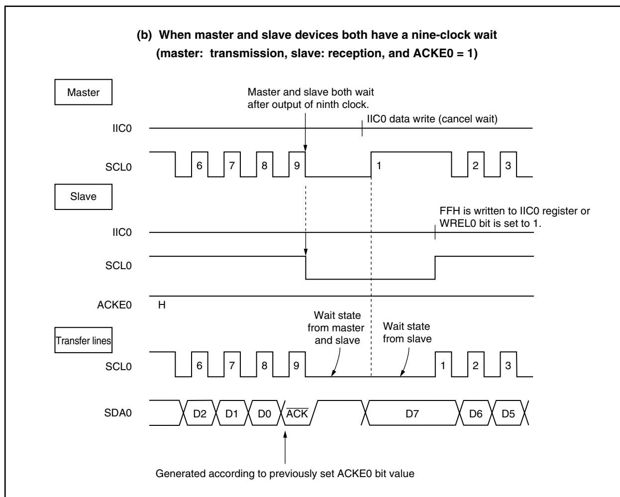
Figure 16-10. Wait State (2/2)
