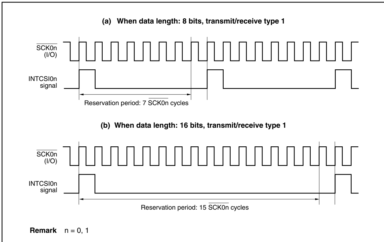
Figure 15-6. Timing Chart of Next Transfer Reservation Period (1/2)
