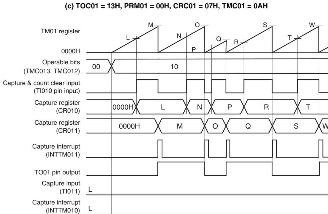
Figure 7-20. Timing Example of Clear & Start Mode Entered by TI010 Pin Valid Edge Input (CR010 Register: Capture Register, CR011 Register: Capture Register) (3/3)
