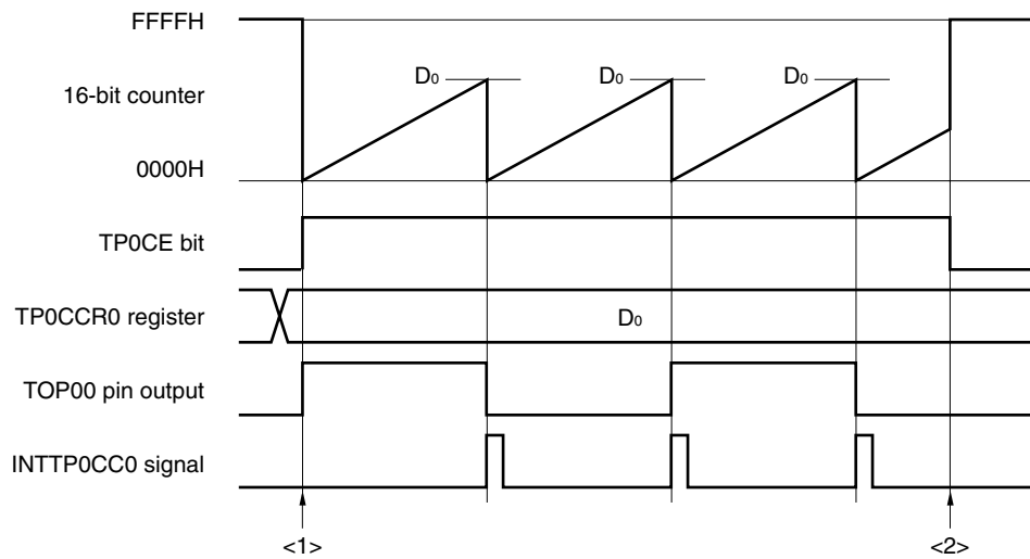
Figure 6-5. Software Processing Flow in Interval Timer Mode
