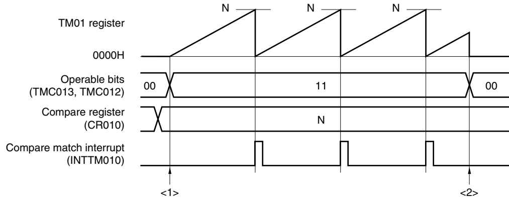
Figure 7-5. Example of Software Processing for Interval Timer Function
