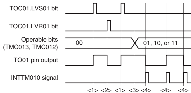
Figure 7-45. Timing Example of LVR01 and LVS01 Bits
