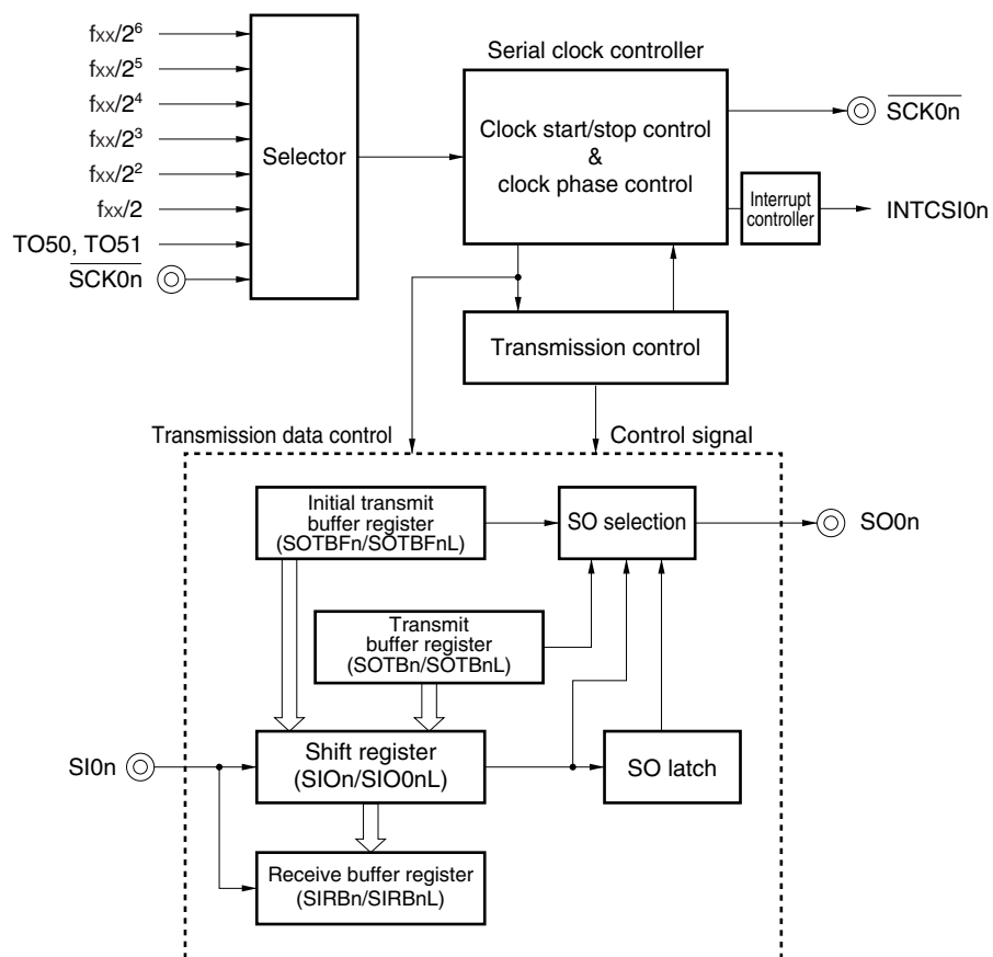
Figure 15-1. Block Diagram of Clocked Serial Interface
