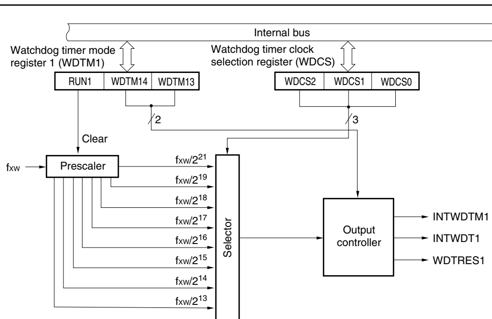
Figure 11-1. Block Diagram of Watchdog Timer 1
