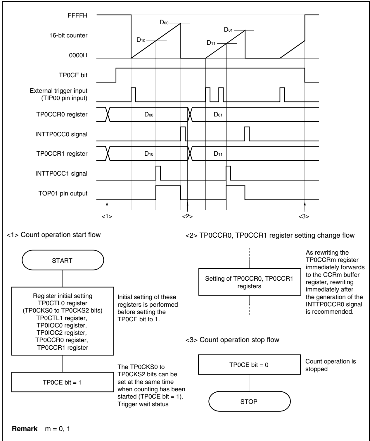
Figure 6-23. Software Processing Flow in One-Shot Pulse Output Mode
