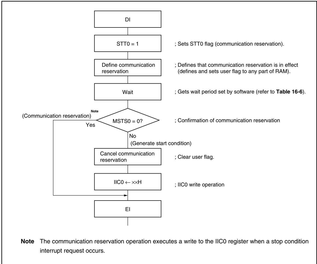
Figure 16-14. Communication Reservation Flowchart
