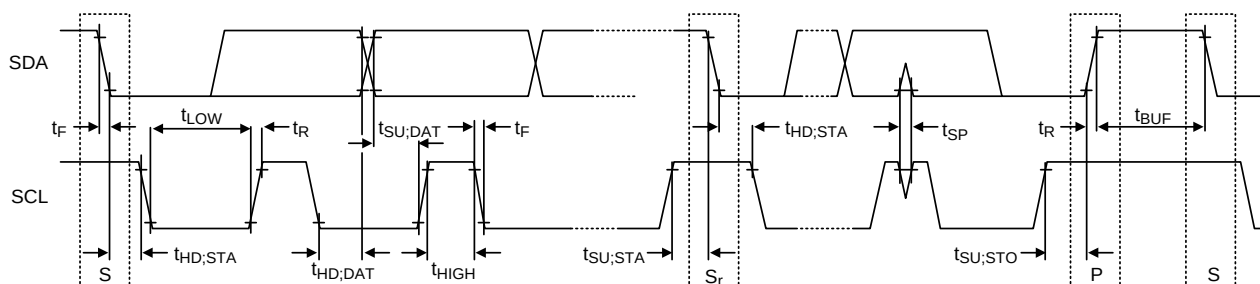
Figure 10. I²C Waveform Information
