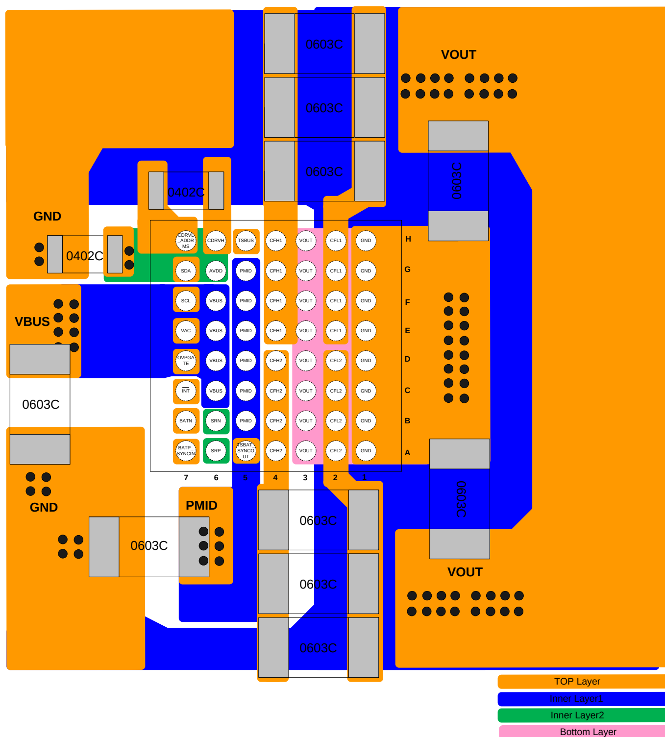
Figure 15. PCB Layout Guide
