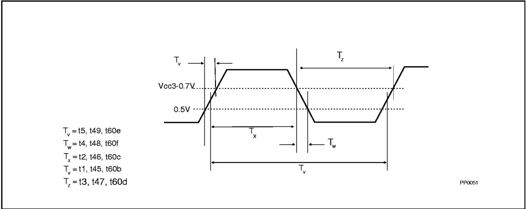
Figure 3. Clock Waveform
