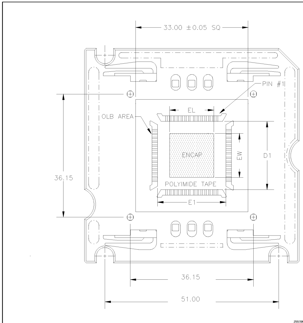
Figure 19. One TCP Site in Carrier (Bottom View of Die)
