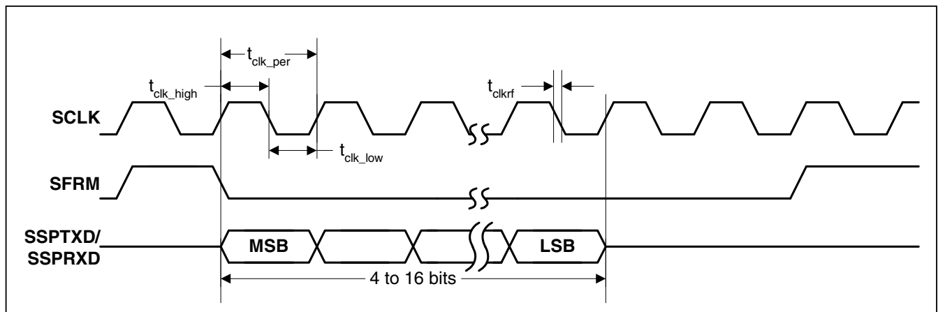
Figure 16. TI Single Transfer Timing Measurement
