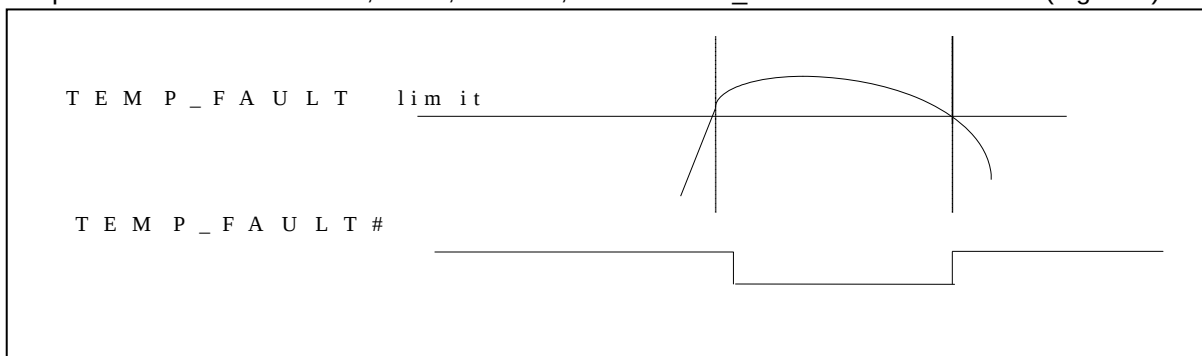
Figure 6. TEMP_FAULT
