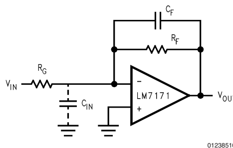
FIGURE 1. Compensating for Input Capacitance
