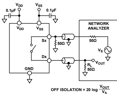
Figure 26. Off Isolation
