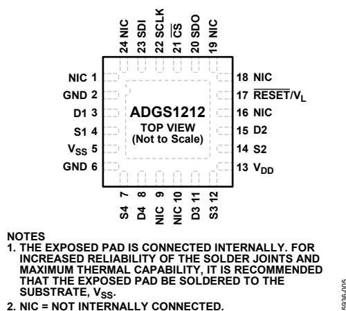
Figure 5. Pin Configuration
