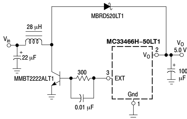
Figure 23. MC33466H-50LT1 Typical Step-Up Application
