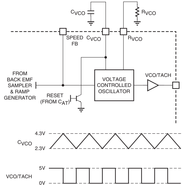
Figure 5. External VCO Component Connections
