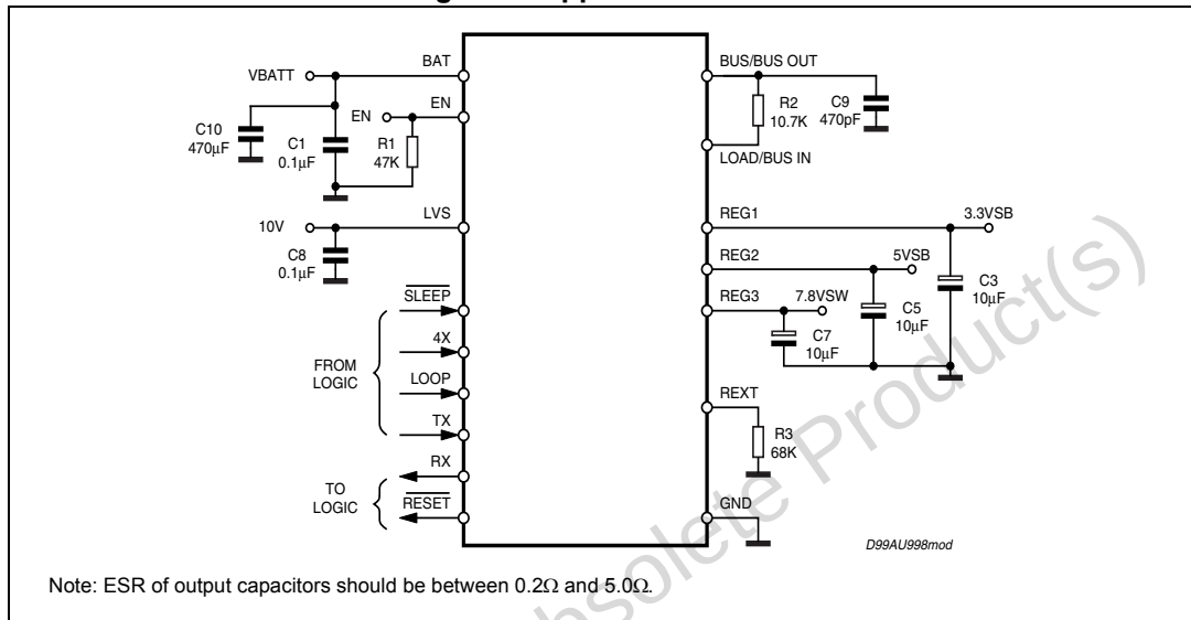
Figure 7. Application circuit
