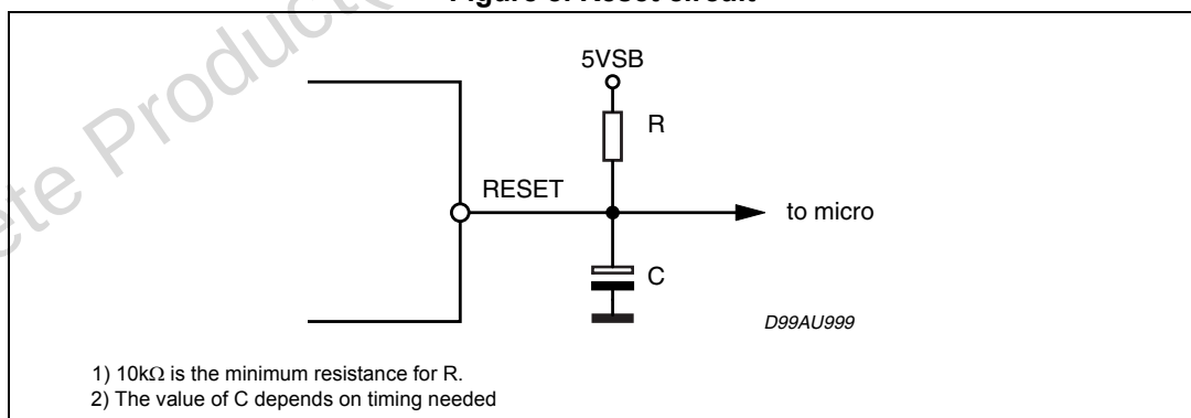
Figure 8. Reset circuit
