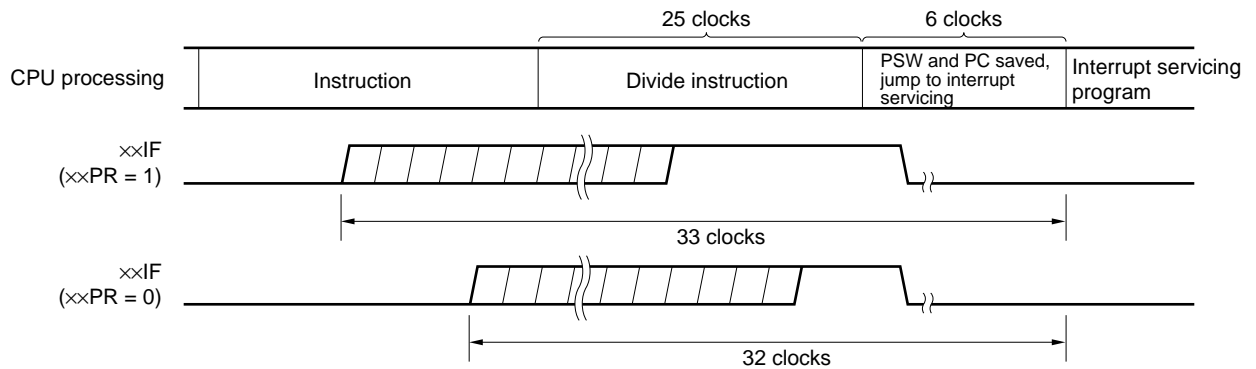
Figure 17-9. Interrupt Request Acknowledgment Timing (Maximum Time)
